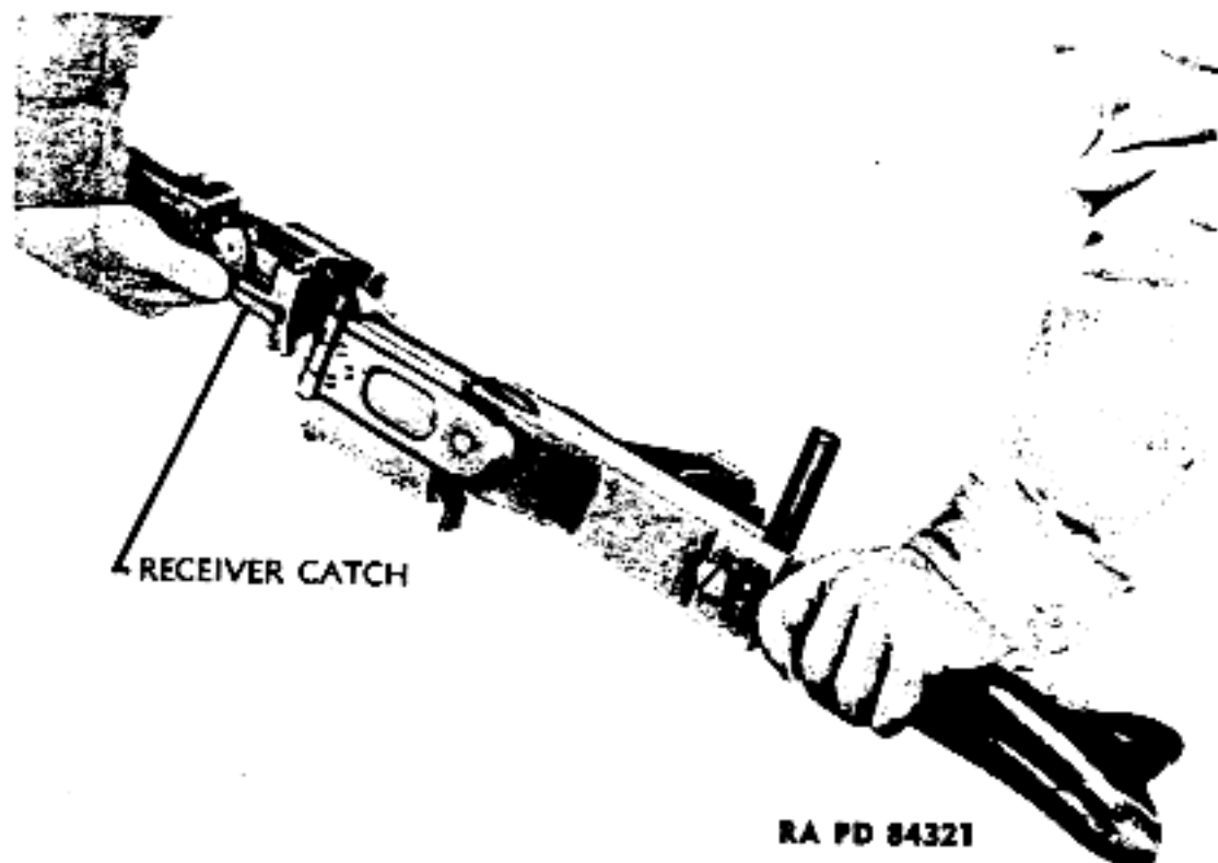
Figure 39 — Unlocking and Rotating Receiver
