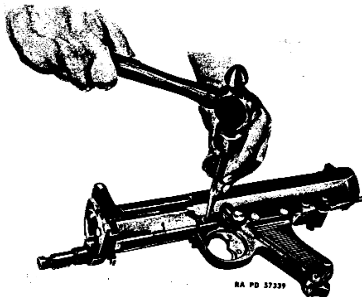
Figure 54 — Removal of Trigger Housing Group
