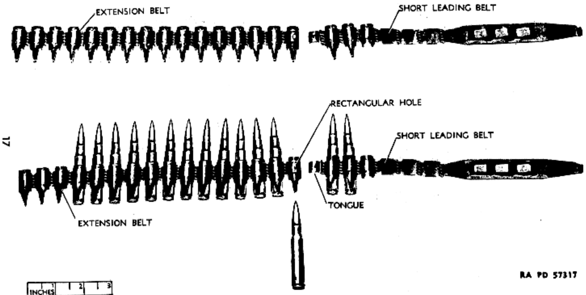
Figure 12 - Loading and Joining of Extension Belt and Short Leading Belt
