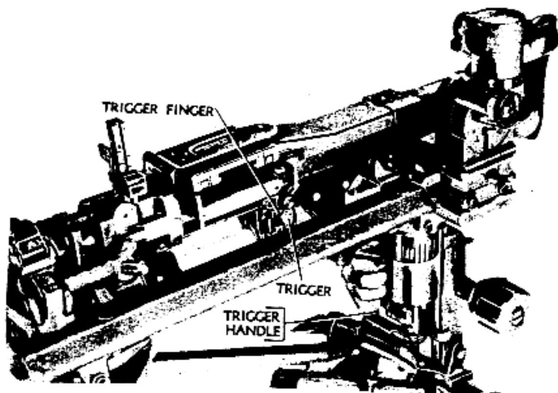
Figure 33 - Firing of Machine Gun
