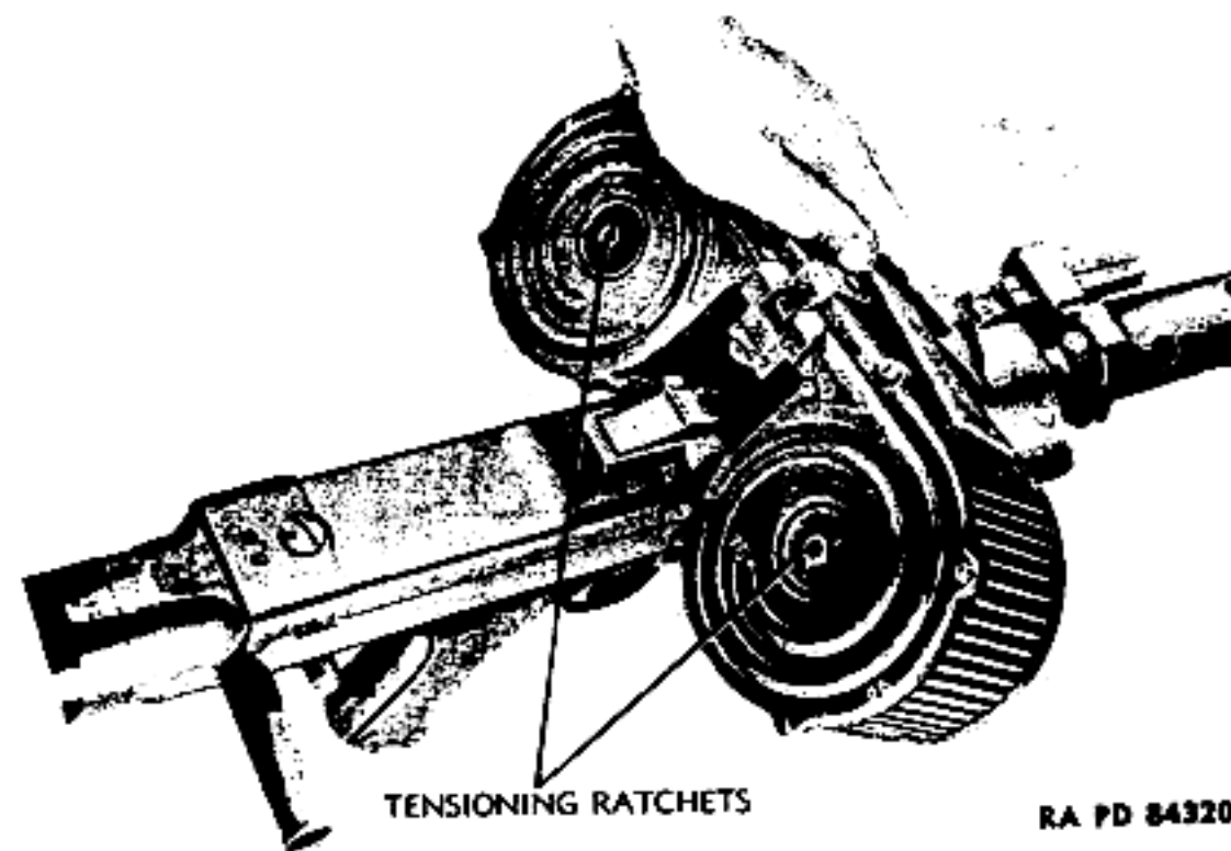
Figure 27 — Mounting of 75-round Magazine
