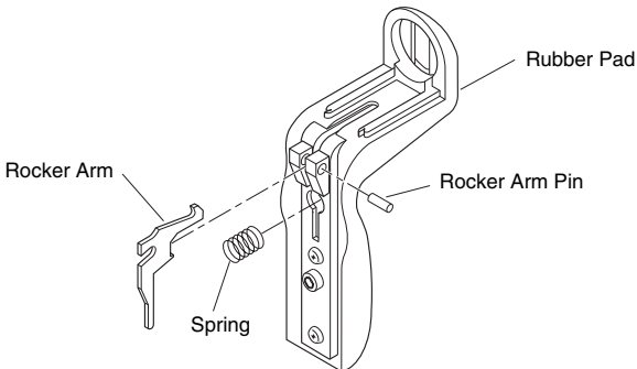
Figure 6 - Removing Rocker Arm
