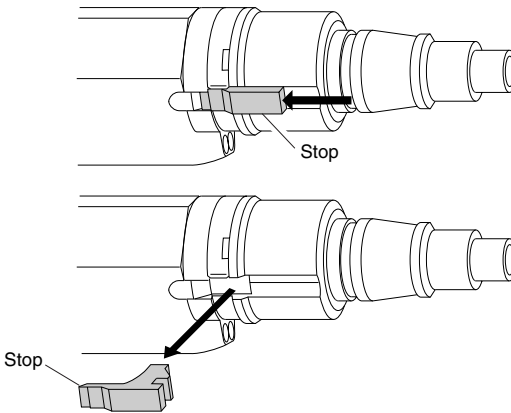
Figure 2 - Removing Stop
