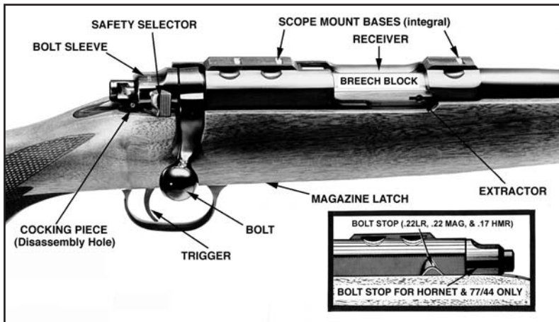
Figure 1. Components frequently referred to are identified. In this illustration the cocking piece is shown cocked (protruding from the rear of the bolt sleeve) revealing the disassembly hole in the lower portion of the cocked piece. The bolt stop (on the left side of the receiver) permits the bolt to be withdrawn simply by pressing down lightly with the thumbnail. The safety selector (shown in the "Fire" position) should be in the "Load-Unload" position when the bolt is being removed or being installed.
