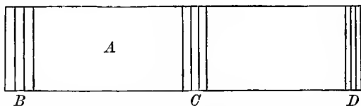
Fig. 46.—A, annealed strip of metal; B, width-keeper for butt; C, same for middle joint; D, same for tip.
