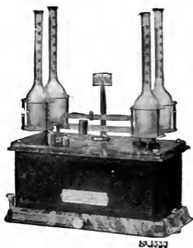
FIG. 35. Torsion balance used for weighing cream in the Babcock test.
