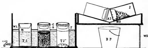
FIG. 46. Cross-section of the Wisconsin curd test, TJ-TJ", testing jars showing different stages of test; WL, water line; M, milk; F, frame; WS, stand to support cover; AI, drain holes; WO, water outlet; DP, drain pail.
