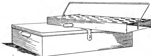
FIG. 58c. Cream sample bottle case.
