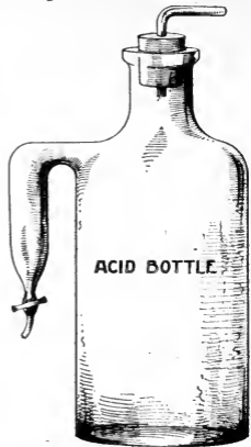
FIG. 18. Acid measuring bottle the side tube is made to hold 17.5 cc. of acid.
