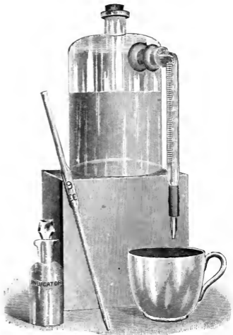
FIG. 44. The Marshall acid test.
