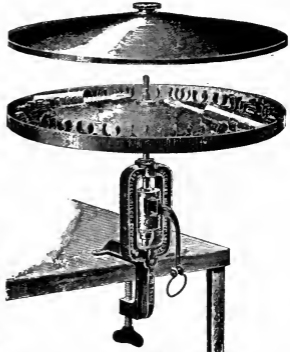
FIG. 1. The Gerber acid-butyrometer.
