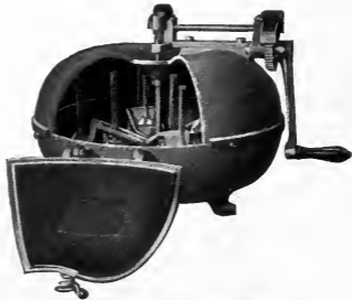
FIG. 21. Type of Babcock hand testers.
