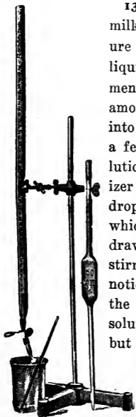
FIG. 41. Apparatus used in Manns' test.
