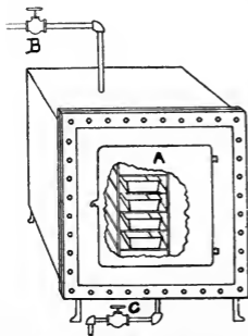
Fig. 60. The Wisconsin high-pressure oven.
