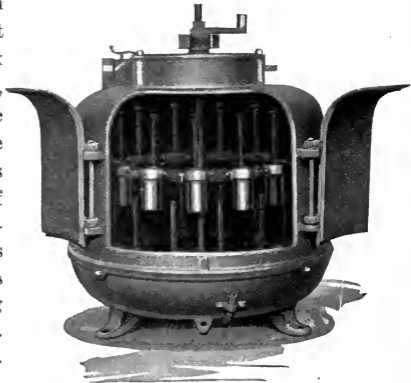
FIG. 23. Type of Babcock steam turbine testers.
