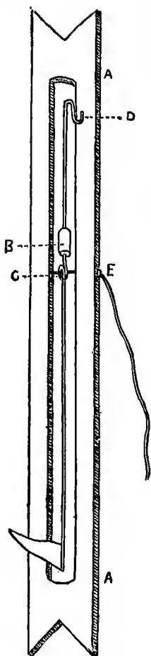
Fig. 74. Improved "Tip-Up."
