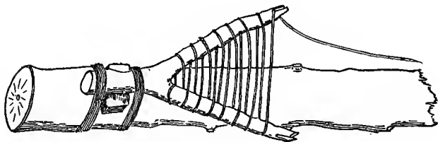
Fig. 1. — Home-made Winder for Pole.
