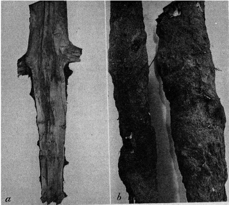
FIG. 25.—(a) Tap-root of young rubber tree affected by brown-root disease. Split open to show fine, brown lines of fungus tissue developed in diseased woody tissues. (b) External appearance of rubber roots attacked by brown-root disease, showing thick, earthy covering encrusting diseased roots.
