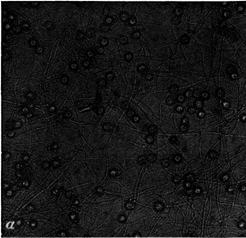
FIG. 34 a.— Pythium complectens . Sporangia and Oogonia of P. complectens developed in pure culture. (Photograph by Mr. R. M. Richards.)
