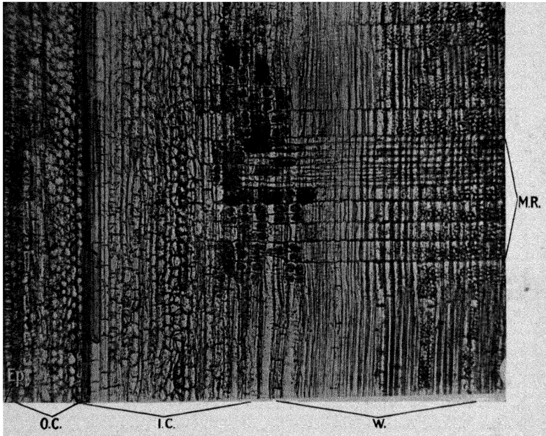
FIG. 4.—Longitudinal radial section of stem.
