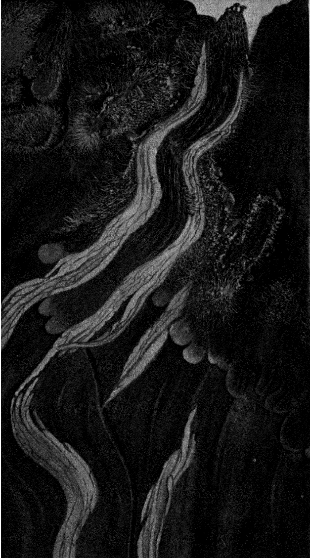
FIG. 13.—Mat of rhizomorphs of S. repens , formed by fusion. Found in diseased cortical tissues of roots. Note mat about to break up at edges into individual rhizomorphs. Also pink spore masses of Stilbum fructifications.
