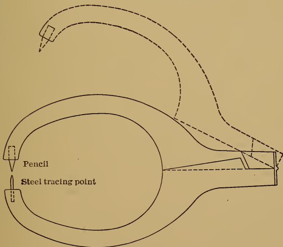
FIG. 25.—Marking Calipers.
