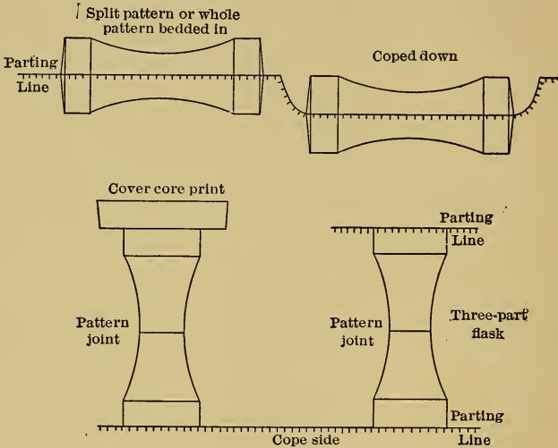
FIG. 6.—Possible Patterns for a Solid Roller.
