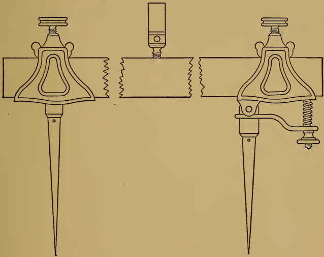
FIG. 13.—Trammel Points.
