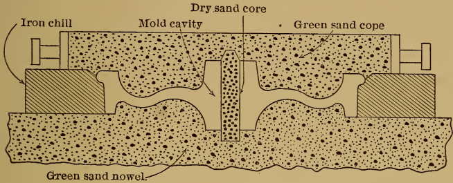
FIG. 3.—Section of Mold with Chill.
