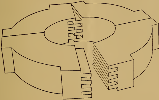
FIG. 65.—Canadian Dovetail.
