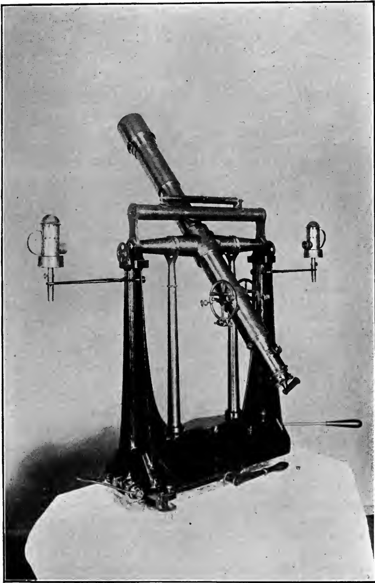
FIG. 48.—Portable Transit.
