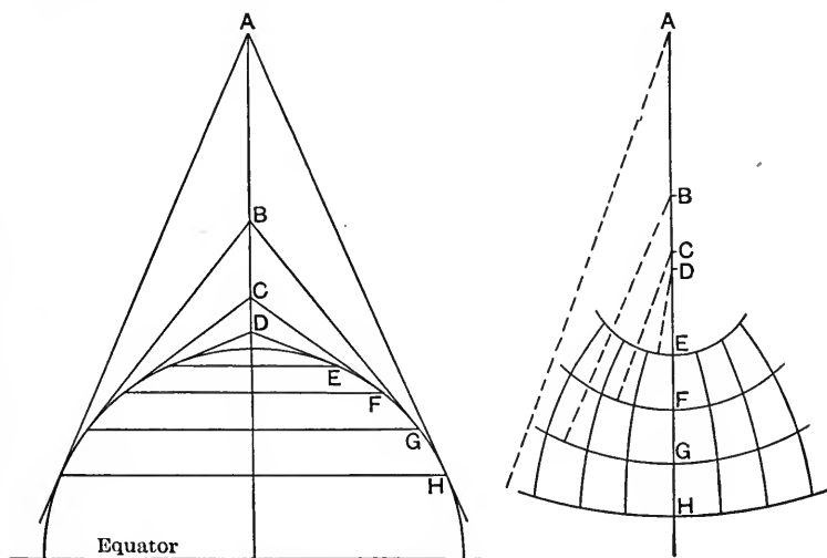
FIG. 62.—Polyconic Projection.
