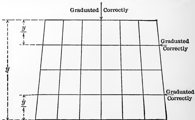
FIG. 57.—Trapezoidal Projection.
