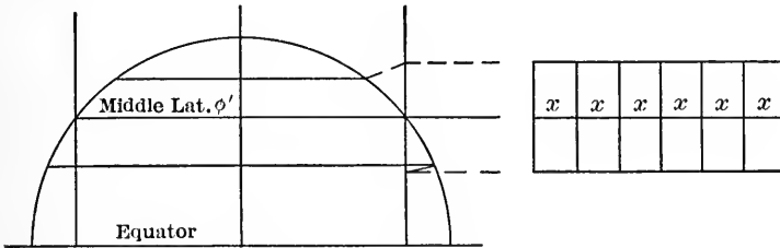
FIG. 55.—Rectangular Cylindrical Projection.
