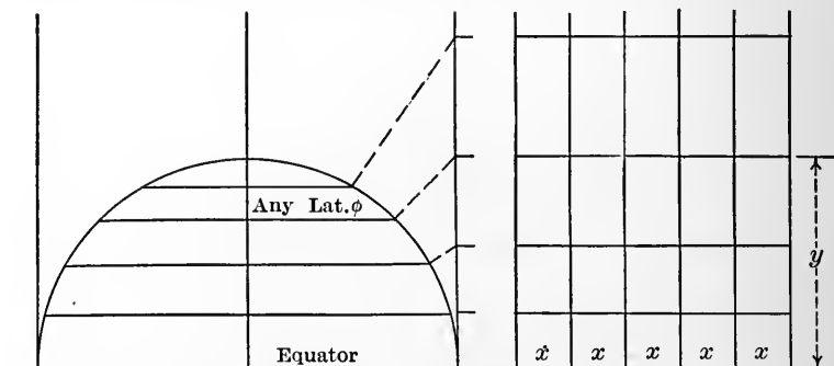
FIG. 56.—Mercator's Cylindrical Projection.
