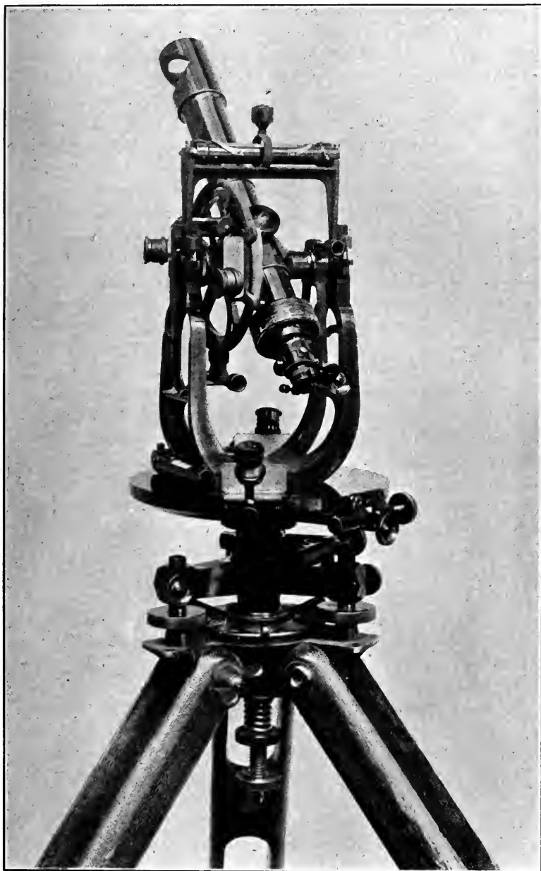
FIG. 18.—Altazimuth Instrument. From a photograph loaned by the U. S. C. and G. S.
