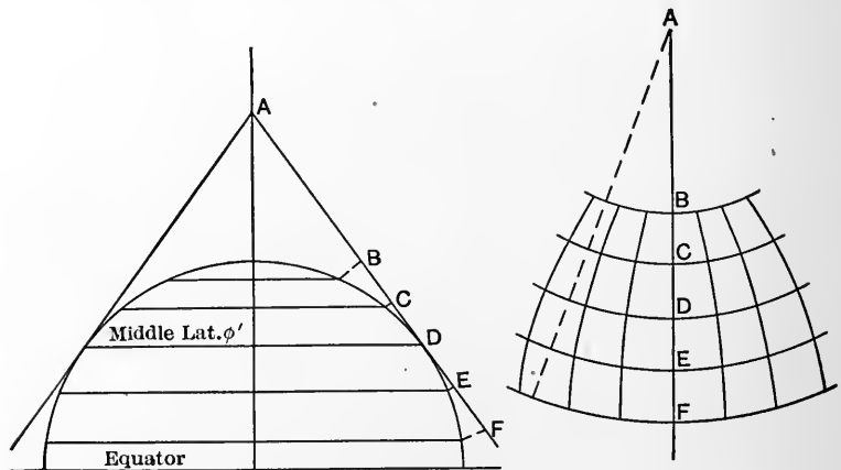
FIG. 61.—Bonne's Conic Projection.
