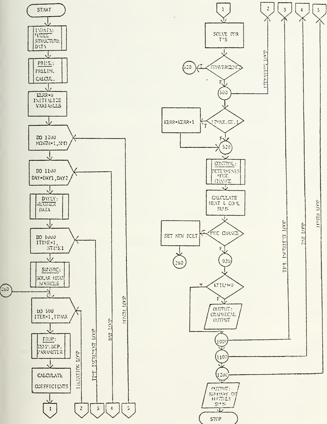
Fig. 1. PASOLE main program.
