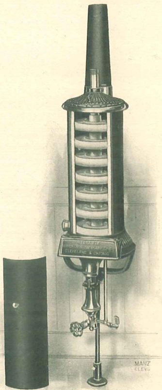
Water Heater with front panel removed, showing inside construction.
