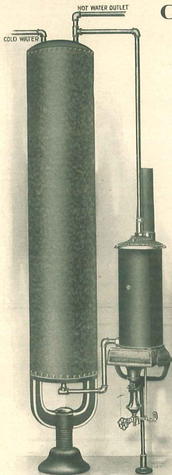
Water Heater connected to kitchen boiler
