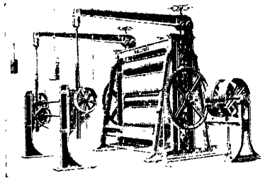
FIG. 24.—Calendering Machine.
