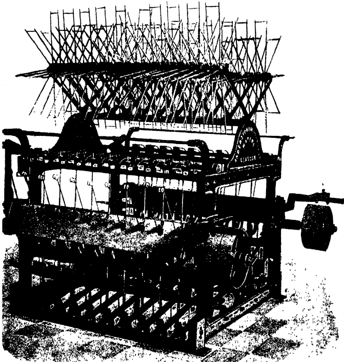
FIG. 8.—Cop Winding Machine to wind from the Hank.
