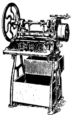
FIG. 16 — Peg and Lace-hole Cutting Machine.
