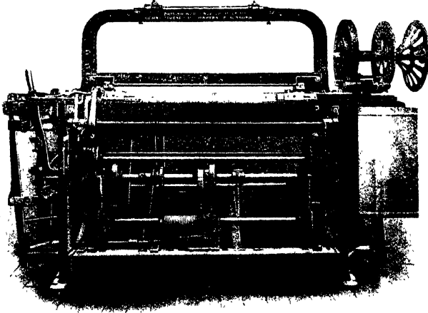
FIG. 20.--Northrop Linen Loom.
