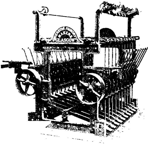
FIG. 7.—Cop Winding Machine to wind from Bobbin.
