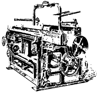
FIG. 10.—Hessian Loom.
