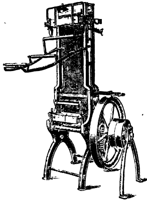
FIG. 17.—Jacquard Card Repeating Machine.
