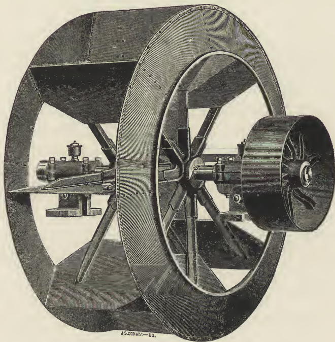
FIG. 140.—Fan wheel.
