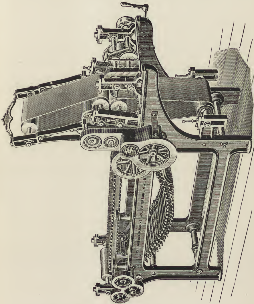
FIG. 42.—Apron head chain-bar drawing frame for Manilla.
