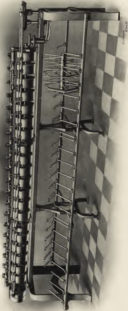
FIG. 81.—Improved single drum winding frame (latch and catch). (Made by Messrs Arundel & Co., Stockport, England.)
