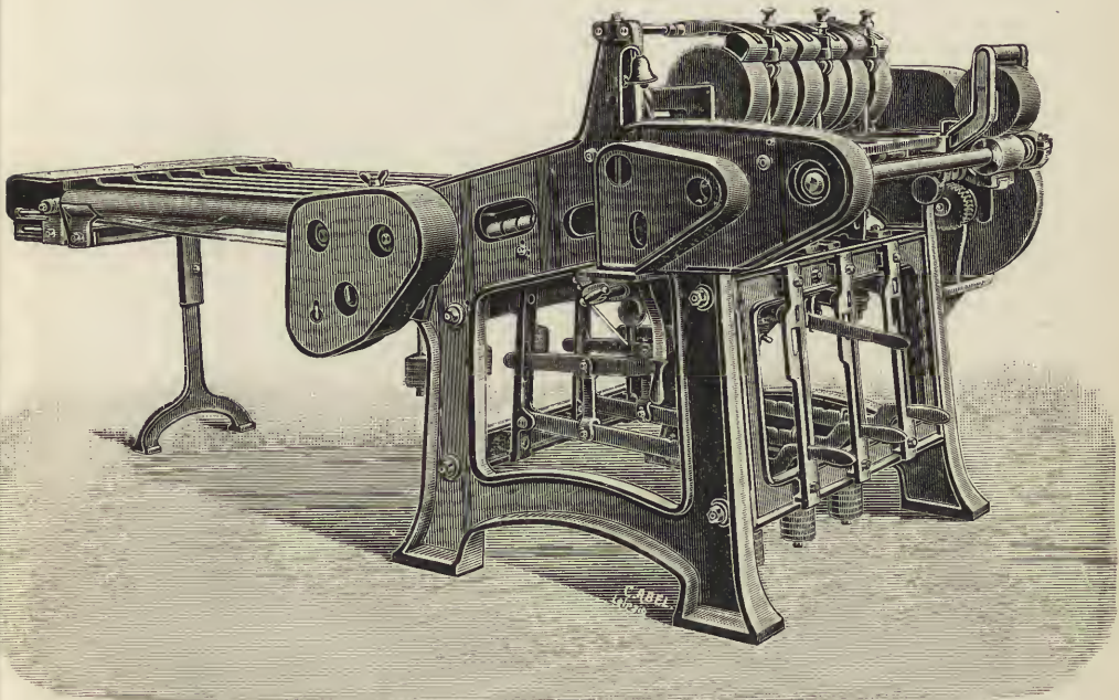
FIG. 23.—Spread-board for flax and hemp. (Made by Oscar Schimmel & Co., Chemnitz, Saxony.)
