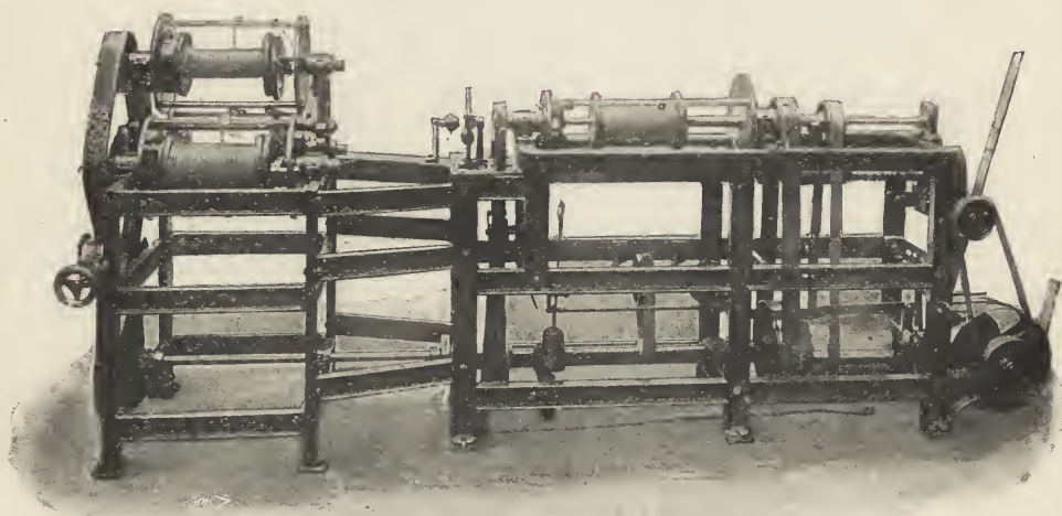
FIG. 90.—Horizontal laying machine for box and sash cords, clothes lines, etc. (2 to 4 fold). (Made by Messrs James Reynolds & Co., Belfast.)
