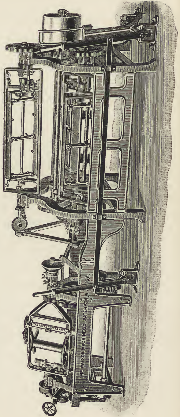
FIG. 127.—Six-thread horizontal rope machine for forming and laying rope from \frac{3}{8} inch to \frac{1}{4} inch in diameter.
