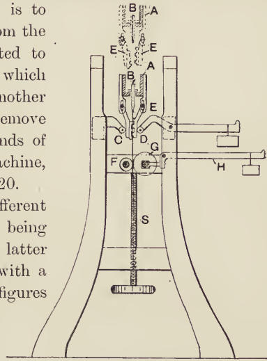
FIG. 19.—Erskine's tender.
