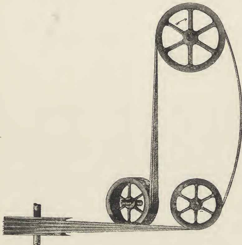
FIG. 160.—Driving with shafts at right angles.
