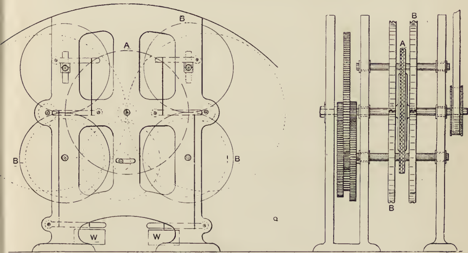
FIG. 8.—Flax cutter.
