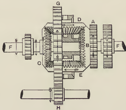
FIG. 52.—Houldsworth's differential motion for the roving frame.
