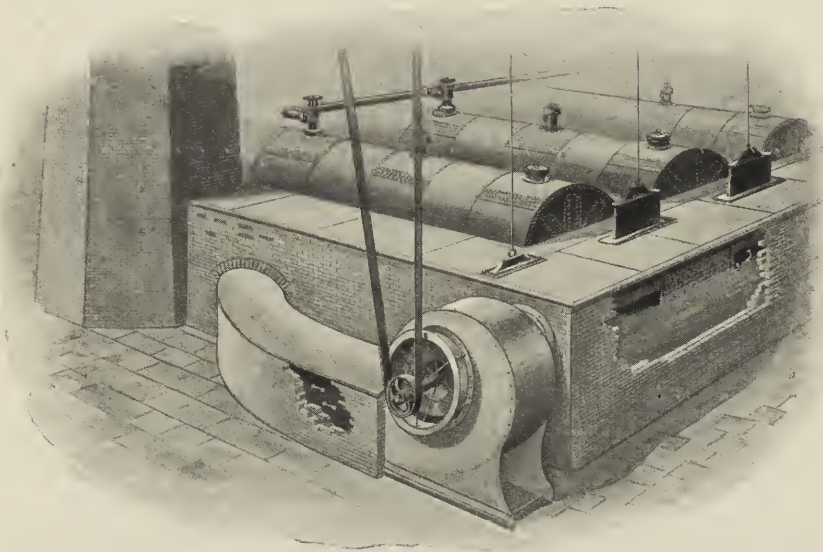
FIG. 153.—Induced draught produced by a Sirocco fan.
