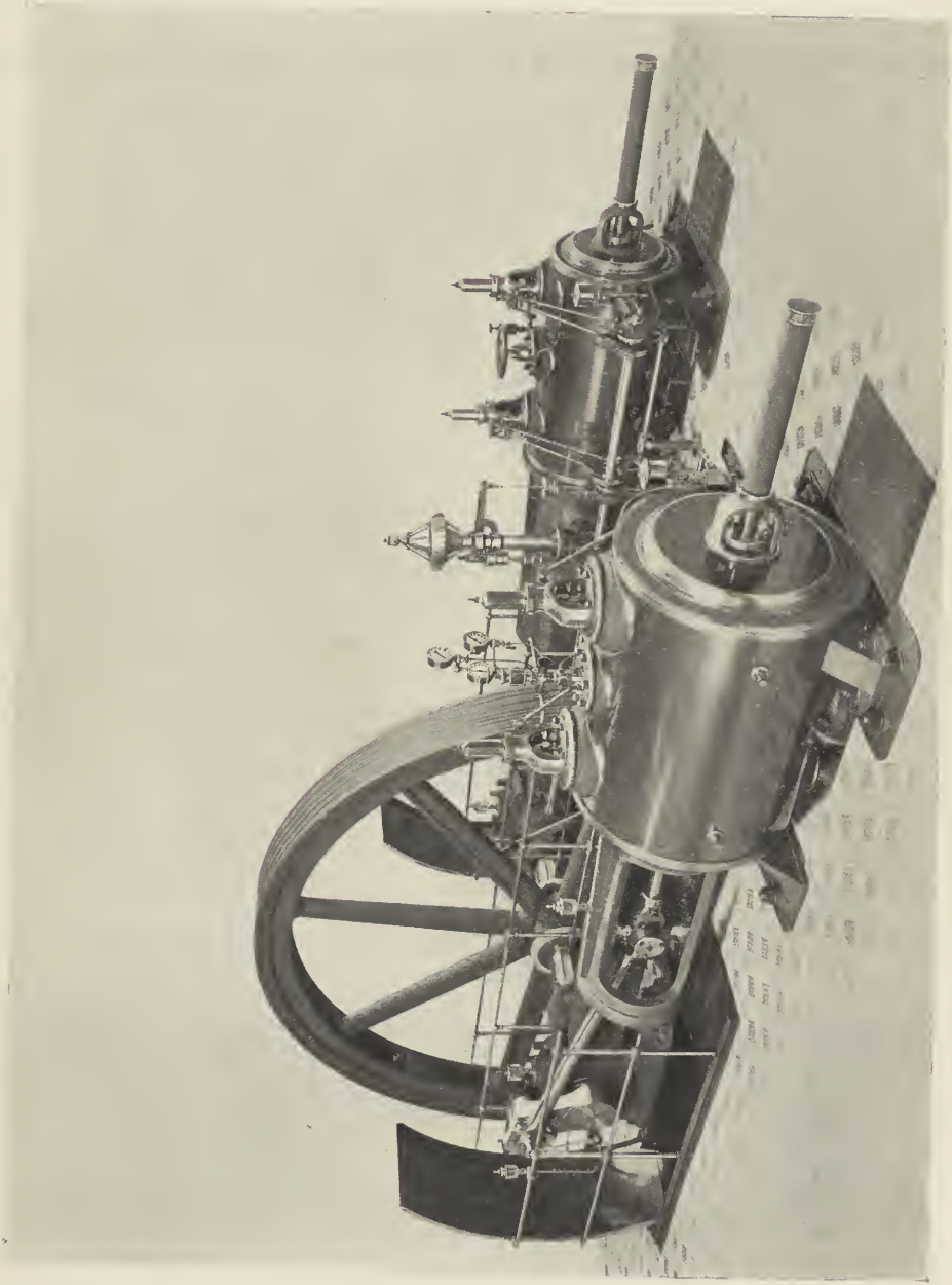
FIG. 155.—Sulzer's horizontal compound mill engine.
