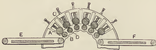
FIG. 7.—Hemp softener.
