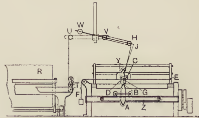
FIG. 74.—Scotch feed.
