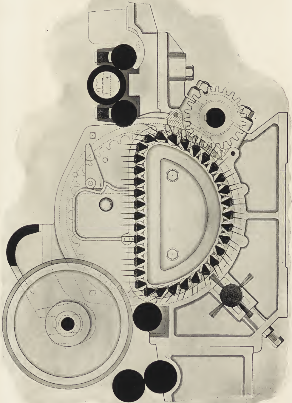
Fig. 45.—Section through bars of Fraser's patent "ring" drawing frame for jute.
