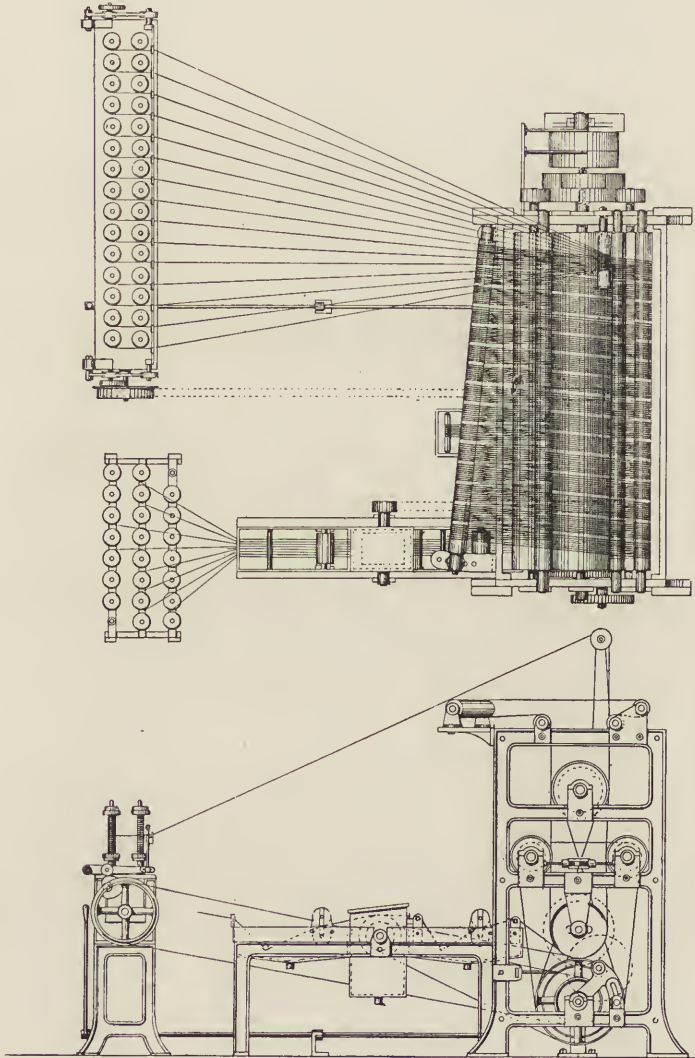
FIG. 93.—Twine polishing machine. (Made by Mr Wm. Bywater, L o eds.)
