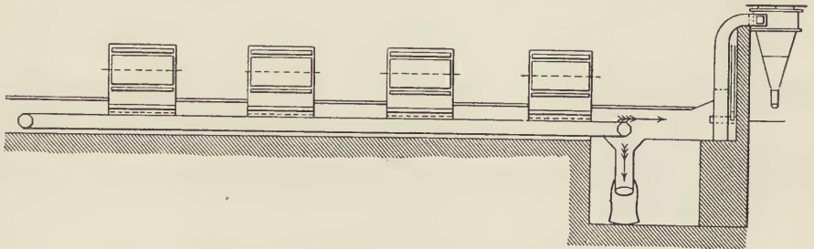
FIG. 143.—Longitudinal section of row of cards with air duct, travelling lattice, dust chambers and cyclone separator.
