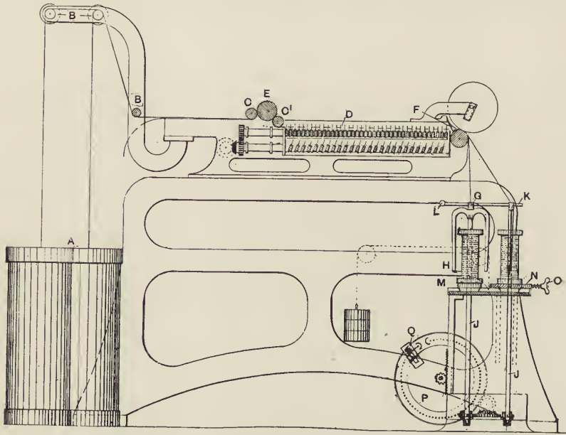
FIG. 50.—Gill spinning frame for rope yarns.
