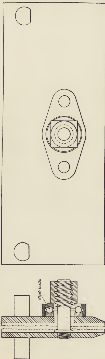
FIG. 15.—Anti-friction washer for hackling machine holder. (Supplied by W. Carter, 28 Waring Street, Belfast.)
