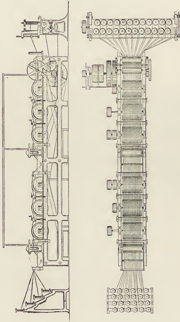
FIG. 92.—Twine twisting and carding machine. (Made by Mr Wm. Bywater, Leeds.)
