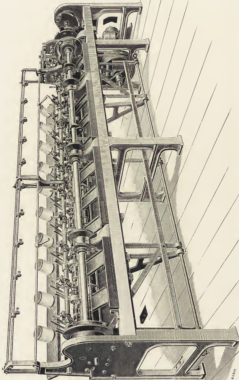
FIG. 111.—New automatic thread spooling machine (Booth's patent).
