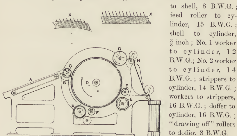
FIG. 31.—Breaker card.
