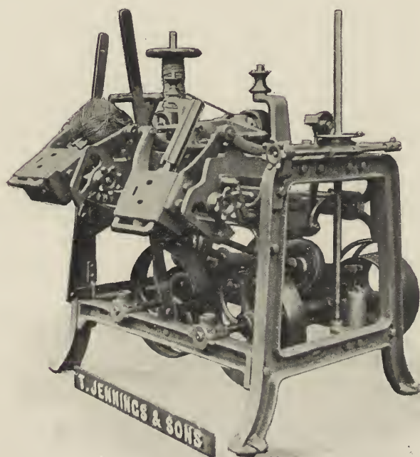
FIG. 79.—Baling machine.
