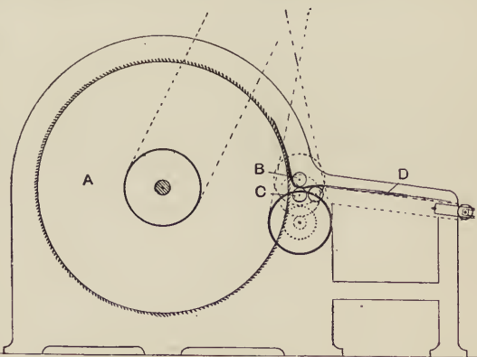
FIG. 4.—Knifing machine.
