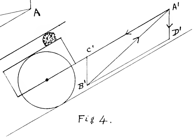
POSITION OF LOAD ON 2 WHEELED VEHICLE.
