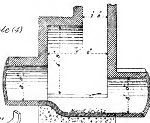
TRANSVERSE SECTION
