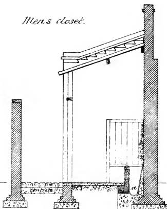
TRANSVERSE SECTION
