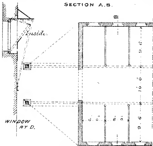
PART PLAN.
