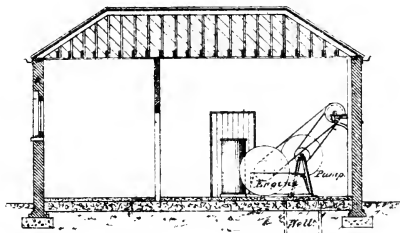
LONGITUDINAL SECTION THRO' ENGINE HOUSE
