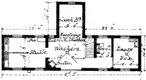
GROUND PLAN.
