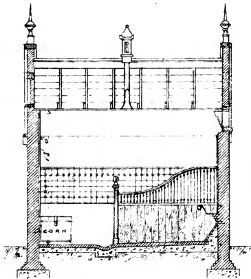
— SECTION ON LINE A. B. —
