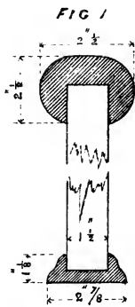
ENLARGED SECTION.
