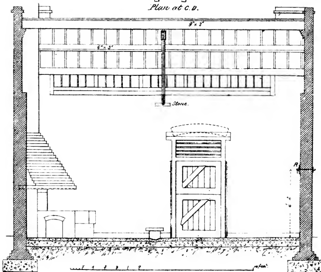
Plan at C.D.
