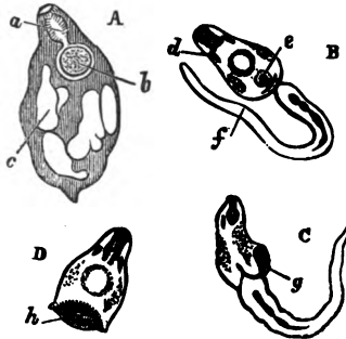
Fig. 5. LARVAL AMPHISTOMES.
