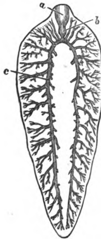
Fig. 2. COMMON FLUKE.
