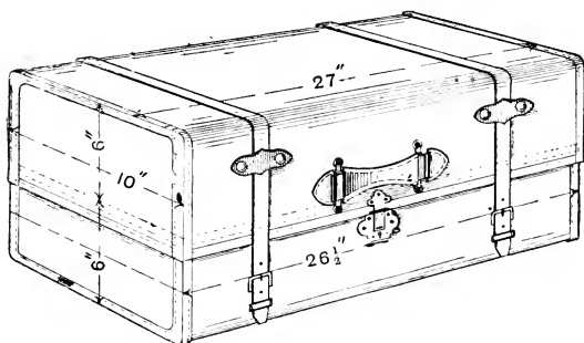
Fig. 96.—Railway Trunk.
