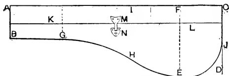
Fig. 61.—Elevation of Mandoline Case.
