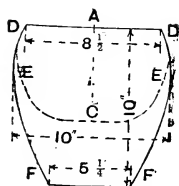
Fig. 71.—Gusset Pattern.
