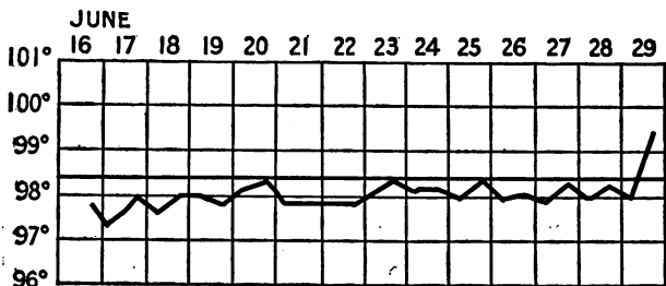
CHART III. Temperature Chart of Entire Squad.
