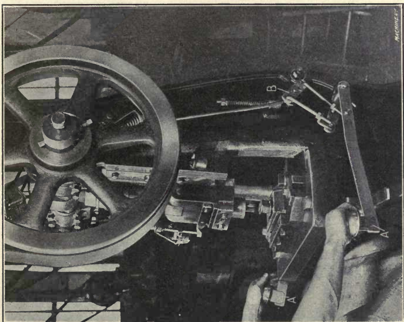
Fig. 20. Arrangement of the Benjamin Stamping Press Guard
