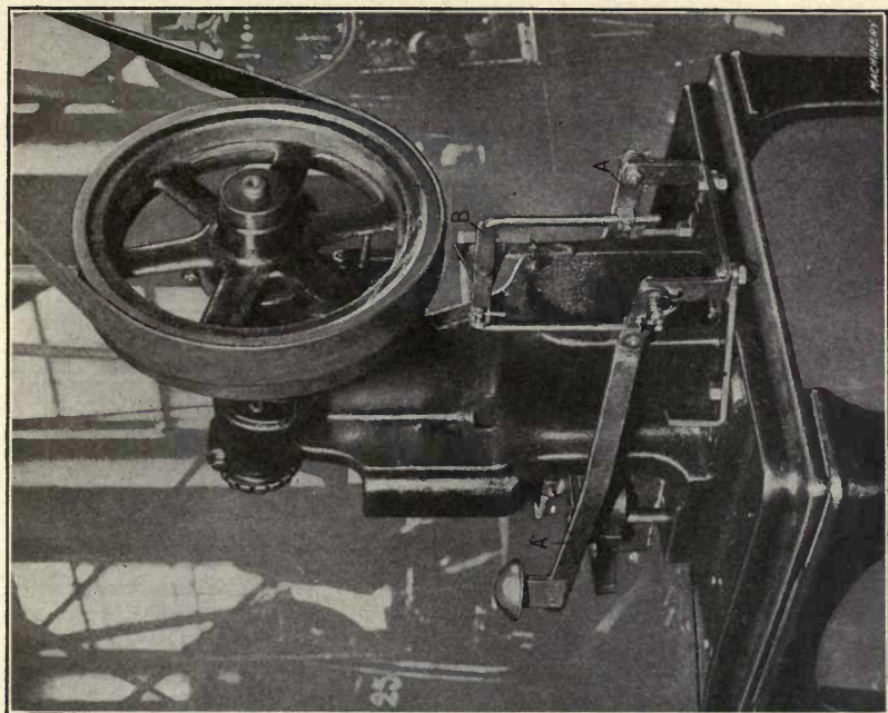
Fig. 21. Another Arrangement of the Benjamin Guard
