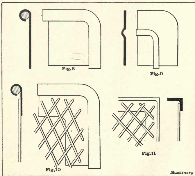
Figs. 8 to 11. Types of Sheet-steel and Wire-mesh Guards
