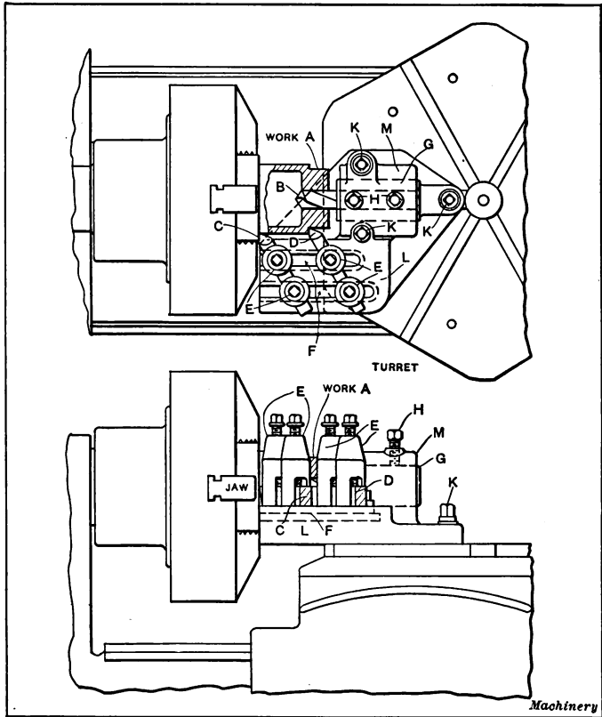
Fig. 2. Multiple Tool-holder for the Turntable Type of Lathe
