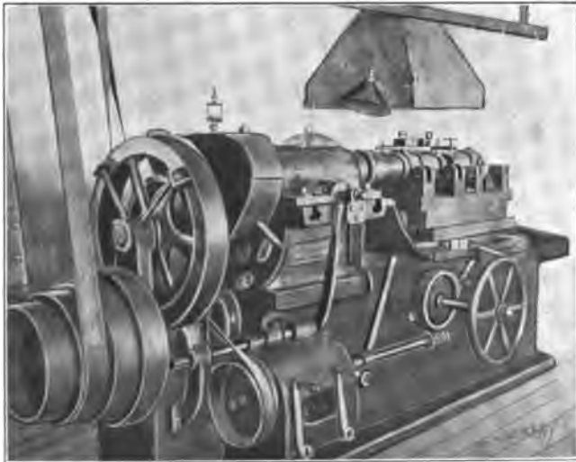
Fig. 25. Boring Cylinders
