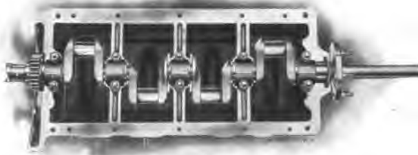
Fig. 19. Top View of Motor Case and Crank-shaft
