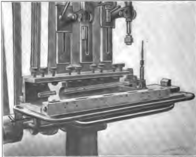
Fig. 24. Fixtures for Drilling and Reaming Cam-shafts
