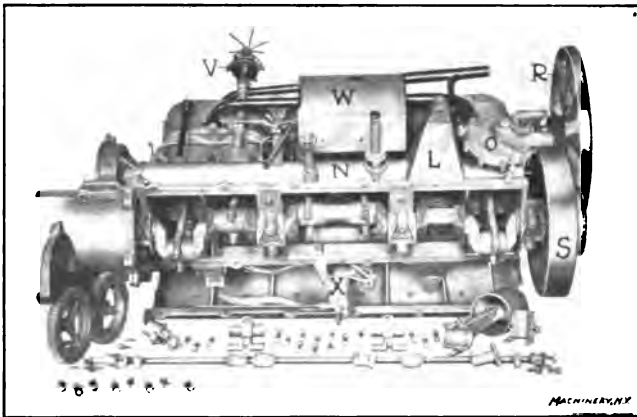
Fig. 6. View of Engine from Beneath, showing Removal of Piston, Cam- and Lay-shafts, etc., without Dismantling
