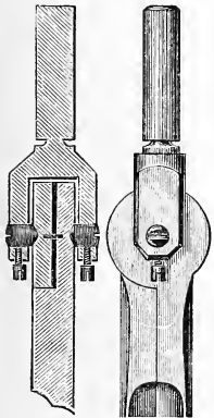
Altener's Patent Joint.
