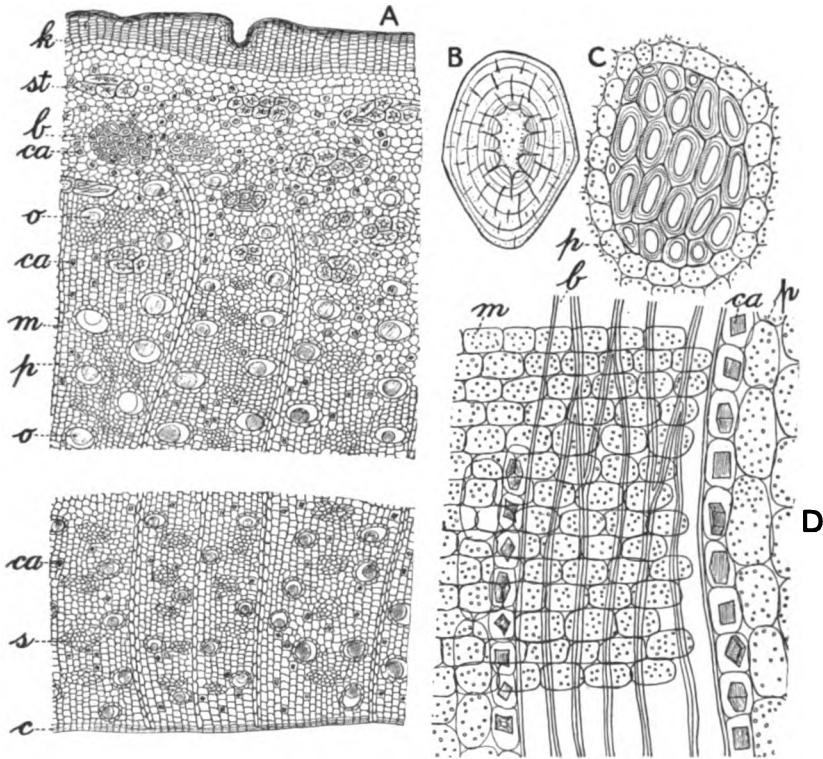
FIG. 238. Southern prickly ash [ Fagara (Xanthoxylum) Clava-Herculis ]: A, transverse section showing cork (k), stone cells (st), groups of primary bast fibers (b), calcium oxalate (ca), medullary rays (m), parenchyma (p) containing starch, oil-secretion reservoirs (o), sieve (s), cambium (c); B, isolated stone cell showing pores and lamellae; C, group of bast fibers found in young, thin bark and surrounding parenchyma (p); D, longitudinal section near a group of bast fibers showing non-lignified bast fibers (b), calcium oxalate (ca) in crystal fibers, medullary rays (m), parenchyma (p) containing starch.
