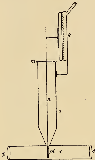
Fig. 189.—Chauveau's hemodromograph (after Langendorff). The tube, p-c , is placed in the course of an artery, the blood after removal of clamps flowing in the direction shown by the arrow. The current strikes the plate, pl , and forces it to an angle varying with the velocity. The movement of pl is transmitted through the stem, n , which moves in a rubber membrane as a fulcrum, m . The angular movement of the projecting end of n may be measured directly or may be made to act upon a tambour, as shown in the figure, and thus be transmitted to a recording drum.
