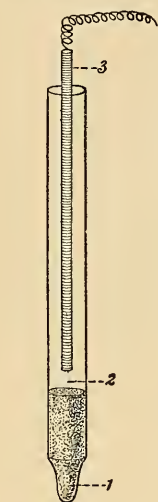
Fig. 44.—To show the structure of a non-polarizable electrode: 1, The pad of kaolin or filter paper moistened with physiological saline (NaCl, 0.7 per cent.) (this is placed on the tissue); 2, the saturated solution of zinc sulphate; (3) the bar of amalgamated zinc.
