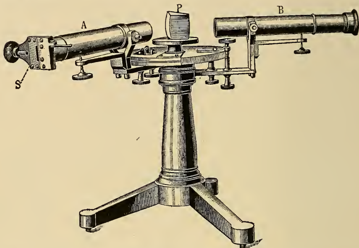
Fig. 182.—Spectroscope: P , The glass prism; A , the collimator tube, showing the slit, S , through which the light is admitted; B , the telescope for observing the spectrum.
