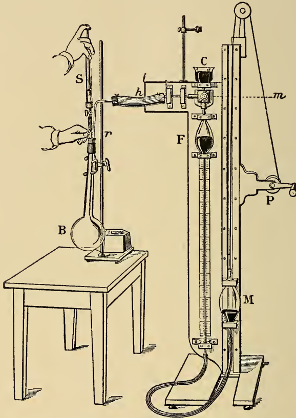
Fig. 272.—Gas pump for extracting the gases of blood ( Gréhant ): M and F , Mercury receivers; P , windlass for raising and lowering M ; m , a three-way stop-cock protected by a seal of mercury or water; C , a cup with mercury over which the receiving eudiometer is placed to collect the gases; B , the bulb in which, after a vacuum is made, the blood is introduced by the graduated syringe, S . By means of the stop-cock m the vacuum in F , caused by the fall of the mercury, can be placed in communication with B . After the gases have diffused over into F , M is raised, and when the stop-cock m is properly turned these gases are driven out through C into the receiving tube. The operation is repeated until no more gas is given off from B .
