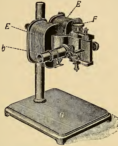
Fig. 42.—One form of the string-galvanometer: E , The electromagnet; b , the projection microscope; F , a screw for varying the tension of the thread.—(Edelmann's Catalogue.)
