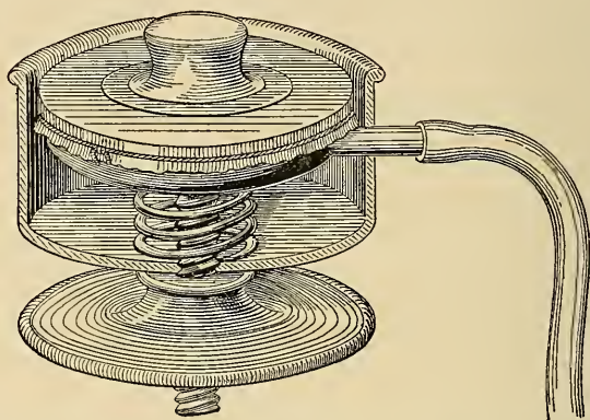
Fig. 228.—Marey's cardiograph. The button on the tambour is pressed upon the chest over the apex. The movements are transmitted through the tube to the right to a recording tambour.
