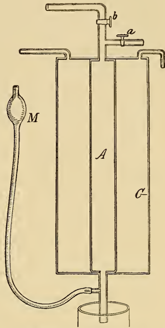
Fig. 274.—Diagram to show the principle of the aerotonometer: A , The tube containing a known mixture of gases, O, CO 2 , N; C , the outside jacket for maintaining a constant body temperature. When stopcock b is open the blood trickles down the sides of A and enters into diffusion relations with the contained gases. After equilibrium is reached the stopcock b is closed and a is opened. By means of the mercury bulb the gases can then be forced out of A into a suitable receiver for analysis.
