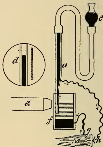
Fig. 41.—Schema of capillary electrometer arranged to show the demarcation current in muscle ( Lombard ): a , The glass tube containing mercury and drawn to a fine capillary below; c , the receptacle containing mercury by raising which the mercury can be driven into the capillary of a ; f , a vessel with glass sides containing mercury below, and above dilute sulphuric acid into which the capillary of a dips; E , the microscope for observing the mercury thread in the capillary; m , the muscle; g and h , the wires touching the longitudinal and cut surfaces of the muscle. The current flows as indicated by the small arrows; d , the capillary thread of mercury as seen under the microscope.
