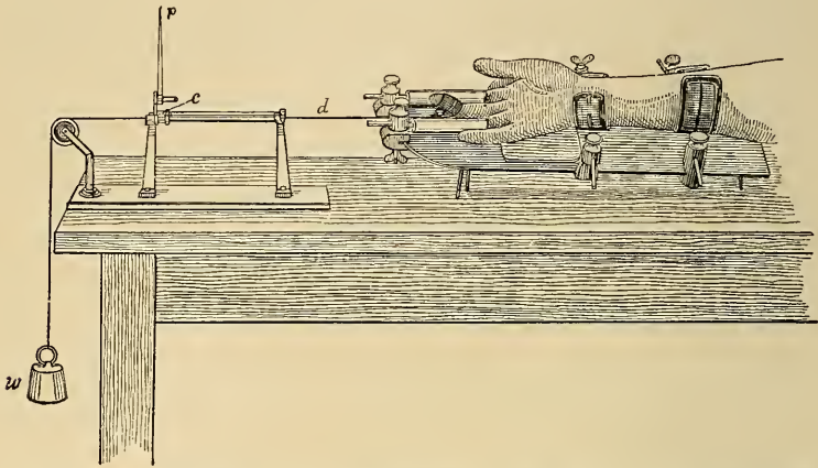
Fig. 23.—Mosso's ergograph: c is the carriage moving to and fro on runners by means of the cord d , which passes from the carriage to a holder attached to the last two phalanges of the middle finger (the adjoining fingers are held in place by clamps); p , the writing point of the carriage, c , which makes the record of its movements on the kymographion; w , the weight to be lifted.
