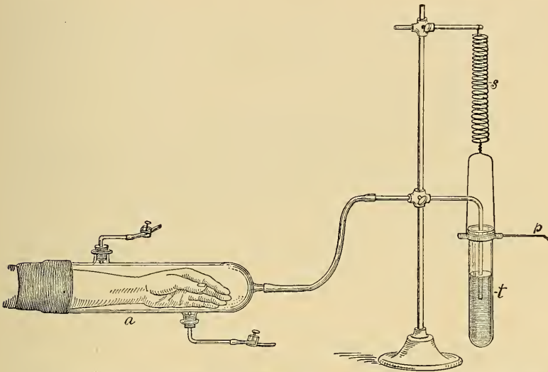
Fig. 249.—A schematic diagram of Mosso's plethysmograph for the arms: a , the glass cylinder for the arm, with rubber sleeve and two tubulatures for filling with warm water; s , the spiral spring swinging the test tube, t . The spring is so calibrated that the level of the liquid in the test tube above the arm remains unchanged as the tube is filled and emptied. The movements of the tube are recorded on a drum by the writing point, p .
