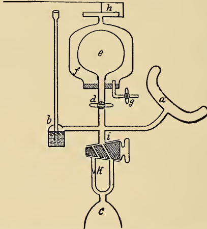
Fig. 203.—Schema showing the construction of the Erlanger apparatus: a , Rubber bag of the arm piece; c , bulb for blowing up this bag and putting pressure on the arm; b , the manometer for measuring the pressure; i , two-way stopcock (when turned so as to communicate with the capillary opening, k , it allows the pressure in a to fall slowly); e , a rubber bag in a glass chamber, f ; e communicates with a when stopcock d is open and the pulse waves from a are transmitted to e ; the pulsations of e in turn are transmitted to the delicate tambour, h , and are thus recorded.
