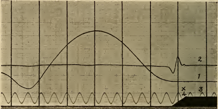
Fig. 48.—Simultaneous record of the mechanical and electrical change in a contracting muscle: 1, Mechanical curve of contraction, photograph of the lever; 2, movement of the string of the string-galvanometer (owing to its faintness it was necessary to retouch this curve); movement upward indicates an increase of negative potential at the upper end of the muscle; 3, time record in hundredths of a second; 4, the stimulating lever; the break in the line indicates the moment of stimulation; on the curve of contraction (1) this moment is indicated by x ; on the curve showing the movement of the string (2) the same instant is marked by the small nick in the curve preceding the large wave caused by the electrical change. The curve was obtained from the gastrocnemius muscle of a frog, stimulated through its nerve by a single induction shock, contraction isotonic. The leading-off electrodes were placed at the ends of the muscle; galvanometer string under tension. The electric curve is diphasic, and both phases are completed within the latent period of contraction ( Snyder ).
