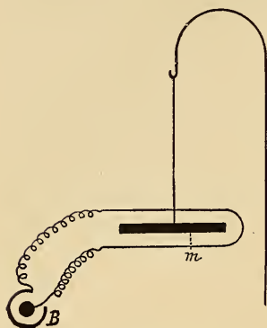
Fig. 38. — Schema showing the principle of construction of the galvanometer: M , The magnet suspended by a thread; B , the battery, with the wires leading off the current encircling the magnet.
