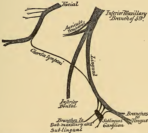
Fig. 289.—Schematic representation of the course of the chorda tympani nerve to the submaxillary gland.
