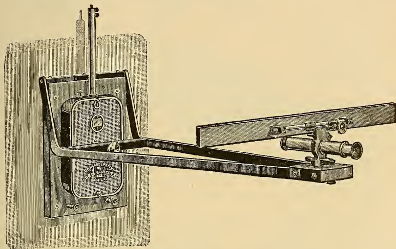
Fig. 39.—D'Arsonval galvanometer as modified by Rowland.
