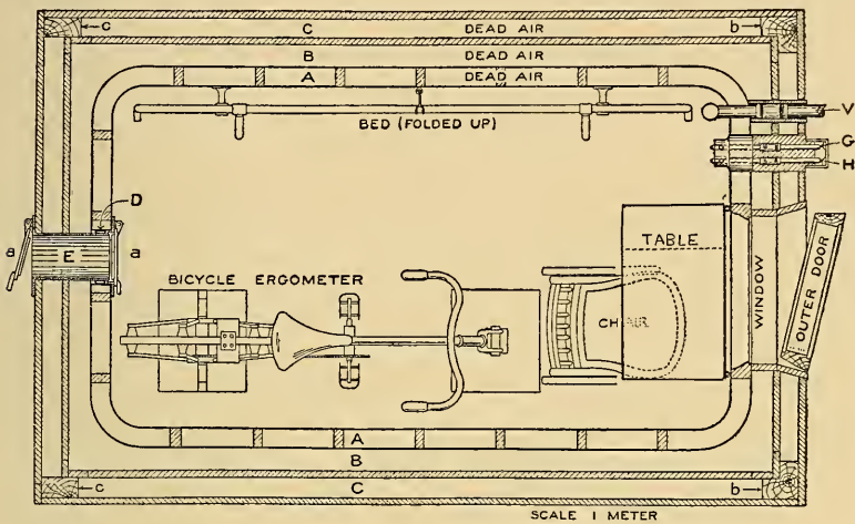
Fig. 301.—Horizontal section of respiration calorimeter. Portions shaded are of wood; A, dead-air space between Cu and Zn walls; B, dead-air space between Zn wall and inside wooden wall; C, dead-air space between inside and outside wooden walls; D, pneumatic-packing air and heat insulated; E, food-aperture tube; a, a, airtight ports (glass); H, ingoing water for absorbing heat; G, outgoing water; V, ventilating air current. (Atwater and Benedict.)
