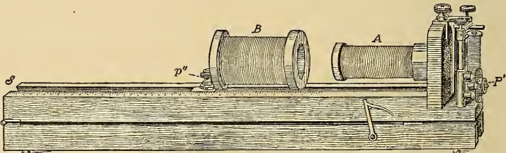
Fig. 6.—The induction coil as used for physiological purposes (du Bois-Reymond pattern): A, The primary coil; B, the secondary coil; P', binding posts to which are attached the wires from the battery, they connect with the ends of coil A; P'', binding posts connecting with ends of coil B, through which the induction current is led off; S, the slide, with scale, in which coil B is moved to alter its distance from A.
