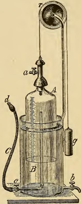
Fig. 268.—Wintrich's modification of Hutchinson's spirometer. —(Reichert.)
