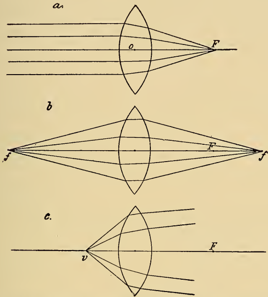
Fig. 124.—Diagrams to illustrate the refraction of light by a convex lens: a., Refraction of parallel rays; b., refraction of divergent rays; c., refraction of divergent rays from a luminous point nearer than the principal focal distance.
