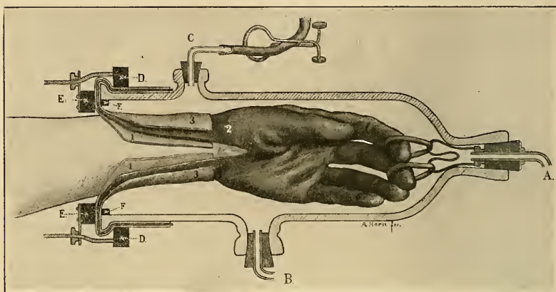
Fig. 250.—Detailed drawing of the glass piezometer with the arrangement of rubber glove to prevent leaking without compressing the veins. 2, The glove with its gauntlet reflected over the end of the glass cylinder; 1 and 3, supporting pieces of stout rubber tubing; D and E, sections of outer and inner rings of hard rubber to fasten the reflected rubber tubing and reduce the opening for the arm.
