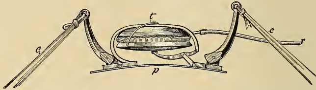
Fig. 266.—Figure of Marey's pneumograph.—(Verdin.) The instrument consists of a tambour ( t ), mounted on a flexible metal plate ( p ). By means of the bands c and c the metal plate is tied to the chest. Any increase or decrease in the size of the chest will then affect the tambour by the lever arrangement shown in the figure. These changes in the tambour are transmitted through the tube r as pressure changes in the contained air to a second tambour (not shown in the figure) which records them upon a smoked drum.
