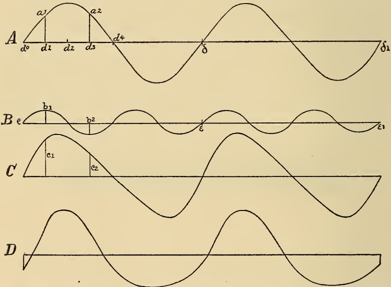
Fig. 175.—Schema by Helmholtz to illustrate the formation of a compound wave from two pendular waves: A and B , pendular vibrations, B being the octave of A . If superposed so that e coincides with d^o and the ordinates are added algebraically, the non-pendular curve C is produced. If superposed so that e coincides with d^i the non-pendular curve D is produced.
