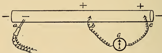
Fig. 46.—Schema to show the arrangement for obtaining a diphasic action current. The arrangement differs from that in Fig. 42 only in that both leading off electrodes, b and c , are placed on the longitudinal surface. No demarcation current is indicated. When the nerve is stimulated at a the negative charge reaches b first, causing a current through the galvanometer from c to b . Subsequently it reaches c and causes a second current in the opposite direction from b to c .
