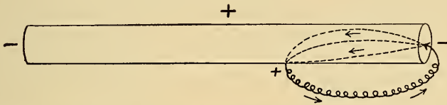
Fig. 37.—Schema showing the course of the demarcation current in an excised nerve, when a point on the longitudinal and one on the cut surface are united by a conductor.
