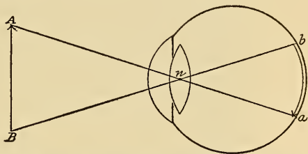
Fig. 128.—Diagram to illustrate the construction necessary to determine the location and size of the retinal image.
