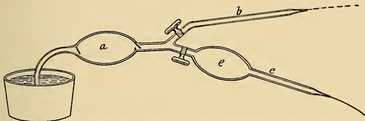
Fig. 210.—Simple schema to illustrate the factors producing a constant head of pressure in the arterial system: a , A syringe bulb with valves, representing the heart; b , glass tube with fine point representing a path with resistance alone, but no extensibility (the outflow is in spurts synchronous with the strokes of the pump); c , outflow with resistance and also extensible and elastic walls represented by the large rubber bag, e ; the outflow is a steady stream due to the elastic recoil of the distended bag, e .
