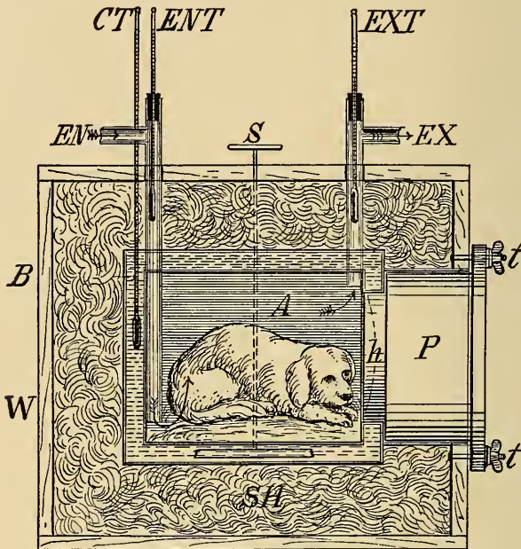
Fig. 300.—Reichert's water calorimeter.
