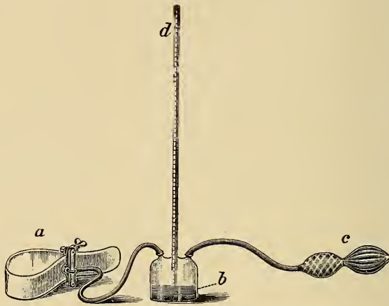
Fig. 201.—Figure of the Riva-Rocci apparatus ( Sahlb ): a , The leather collar with inside rubber bag to go on the arm; c , the bulb for blowing up the rubber bag and thus compressing the artery; d , the manometer dipping into the reservoir of mercury, b , to measure the amount of pressure.
