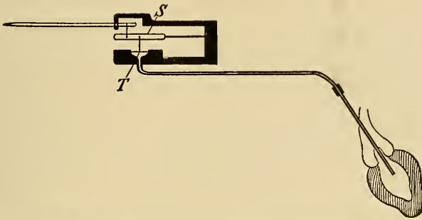
Fig. 196.—Diagram showing construction of Hürthle's manometer.—(After Curtis.) The interior of the heart or the artery is connected by rigid tubing to a very small tambour, T . The tubing and the tambour are filled with liquid. The movements of the rubber dam covering the tambour are greatly magnified by a compound lever, S . The tendency of this lever to "fling" may be prevented by an arrangement not shown in the diagram. The essential principles of the recorder are, first, liquid conduction from heart to tambour; second, a very small tambour and membrane so that a minimal volume of liquid escapes from the heart into the tambour.
