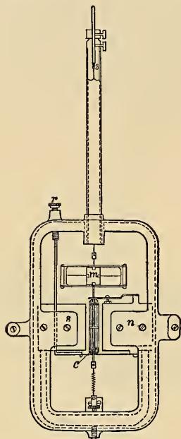
Fig. 40.—Diagram of structure of the d'Arsonval galvanometer. c is the coil of fine wire through which the current is passed. It is swung by a fine thread of phosphor-bronze so as to lie between and close to the poles—( n ) north pole, and ( s ) south pole—of the magnet. Just above the magnet the thread carries a mica or aluminum vane to which is attached a small mirror. The scale of the instrument is reflected in this mirror and is observed through the telescope shown in Fig. 38.
