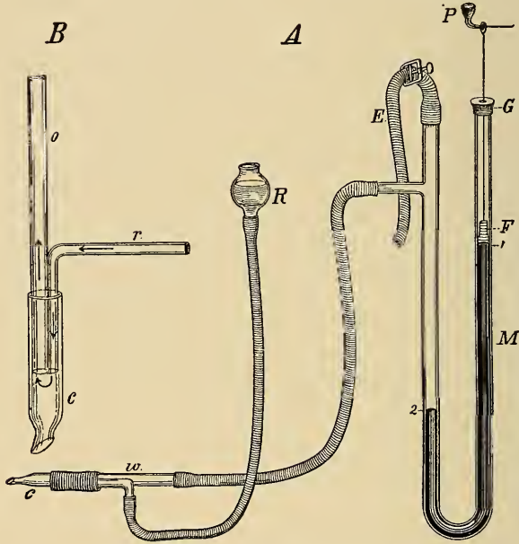
Fig. 192.— A , Schema to show the recording mercury manometer and its connection with the artery: M , The manometer with the position of the mercury represented in black (the pressure is given by the distance in millimeters between the levels 1 and 2; one-half of this distance is recorded on the kymographion by the pen, P ); F , the float resting upon the surface of the mercury; G , the cap through which the stem carrying the pen moves; E , offset for driving air out of the manometer and for filling or washing out the tube to the artery; R , the receptacle containing the solution of sodium carbonate; c , the cannula for insertion into the artery; w , the washout arrangement shown in detail in B .
