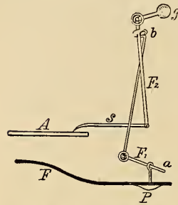
Fig. 213.—The lever of the Dudgeon sphygmograph: P , The button of the spring F , to be placed upon the artery. The movement is transmitted to the lever, F 1 , and thence to the bent lever, F 2 , whose movement is effected through the weight, g . The writing point s , of this lever makes the record on the smoked surface, A .
