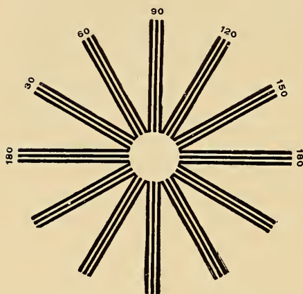
Fig. 134.—Astigmatic chart.
