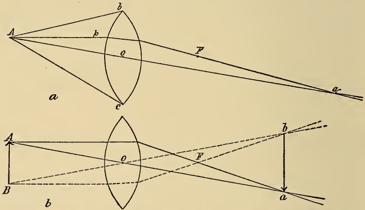
Fig. 125.—Diagrams to illustrate the formation of an image by a biconvex lens: a , Formation of the image of a point; b , formation of the images of a series of points.
