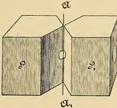
Fig. 43.—Schema to show the relation of the thread to the magnets in the string-galvanometer: AA , The delicate thread of silvered quartz or of platinum, stretched between the polar pieces ( PP ) of an electromagnet. When a current passes through AA , the thread shows a movement. The ends of the magnets are pierced by holes, seen in P 1 , through which the movements of the thread may be watched by means of a microscope or be projected upon a photographic plate.—(After Eindhoven .)
