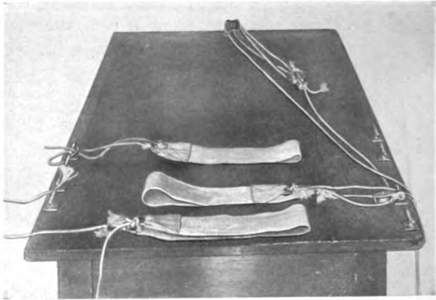
Fig. 380.—Stretching board with loops ready for application to a left dorsal curve (Lovett).
