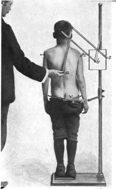
Fig. 346.—Making a tracing of the lateral deviation by the author's scoliosimeter: a , Pointer which follows the line of the spinous processes and tips of the scapulæ; b , pencil recording the tracing on paper to the scale of 1 to 4; c , fixed point of the pantograph.
