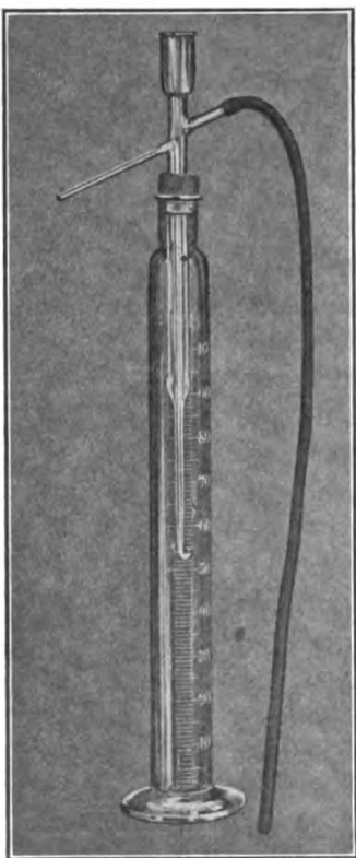
FIG. 121.—CROLL'S FAT APPARATUS.
