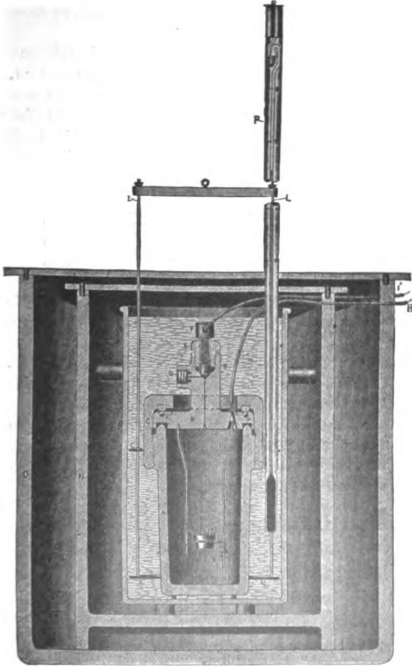
FIG. 185.—BERTHELOT-ATWATER BOMB CALORIMETER.
