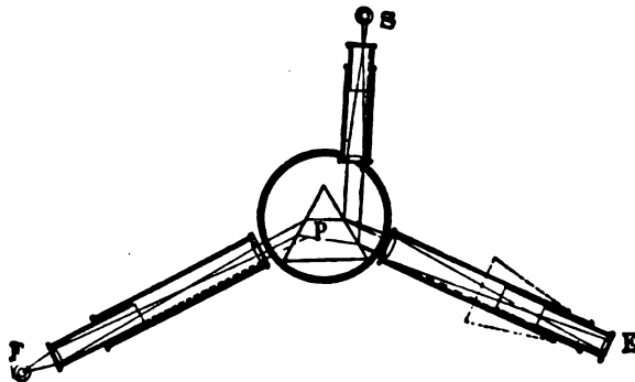
FIG. 94.—DIAGRAM OF ANGULAR-VISION SPECTROSCOPE. (Long.)
