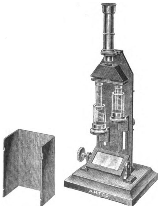
FIG. 168.—DUBOSCQ COLORIMETER.
