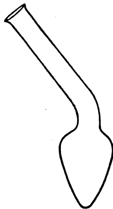
FIG. 172.—GULICK MICRO-OXIDATION FLASK.
