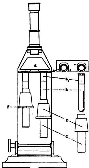
FIG. 89.—BLOOR'S NEPHELOMETER.
