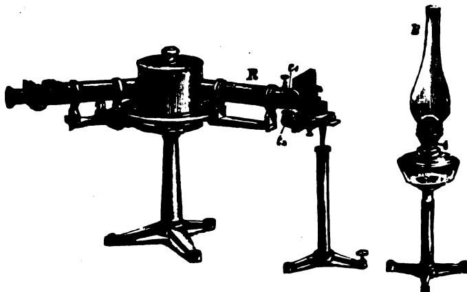
FIG. 93.—ANGULAR-VISION SPECTROSCOPE ARRANGED FOR ABSORPTION ANALYSIS.
