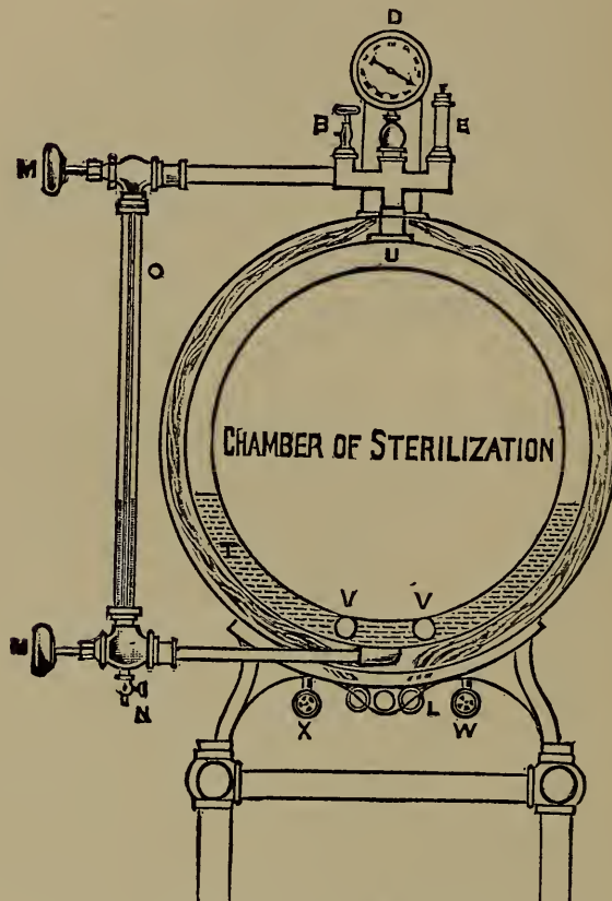
Steam-sterilizer (in section).
