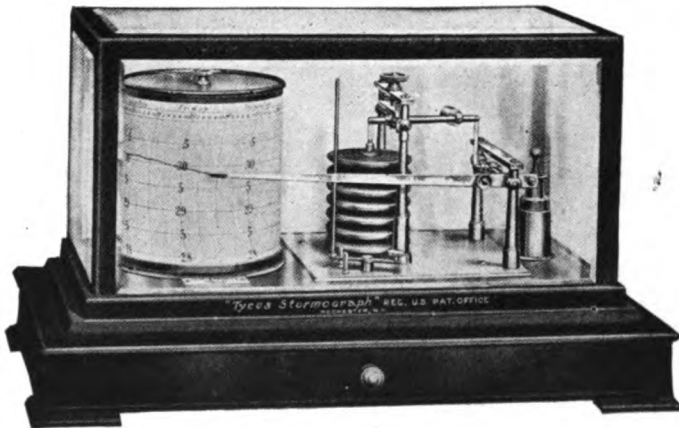
Barograph.
