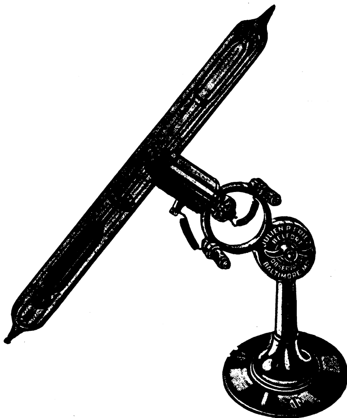
Sunshine differential thermometer, electrically connected with the recording apparatus.
