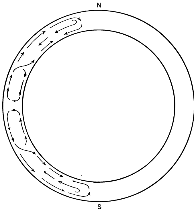
Convectional movements of the air; sectional view.
