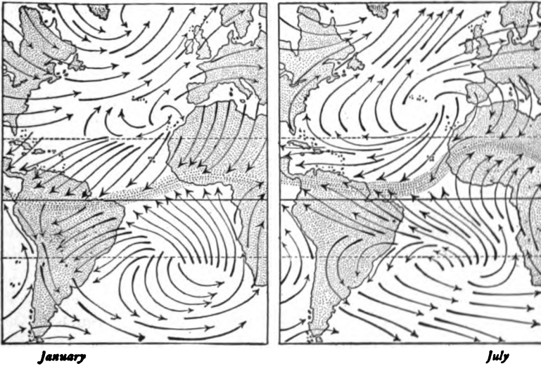
Winds of the Atlantic.
