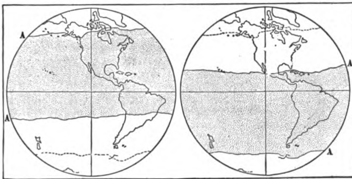
The migration of the heat belt.
