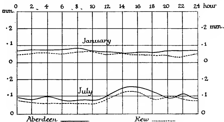
Fig. 65.—Diurnal Variation in Rainfall—Period 1871-1910
