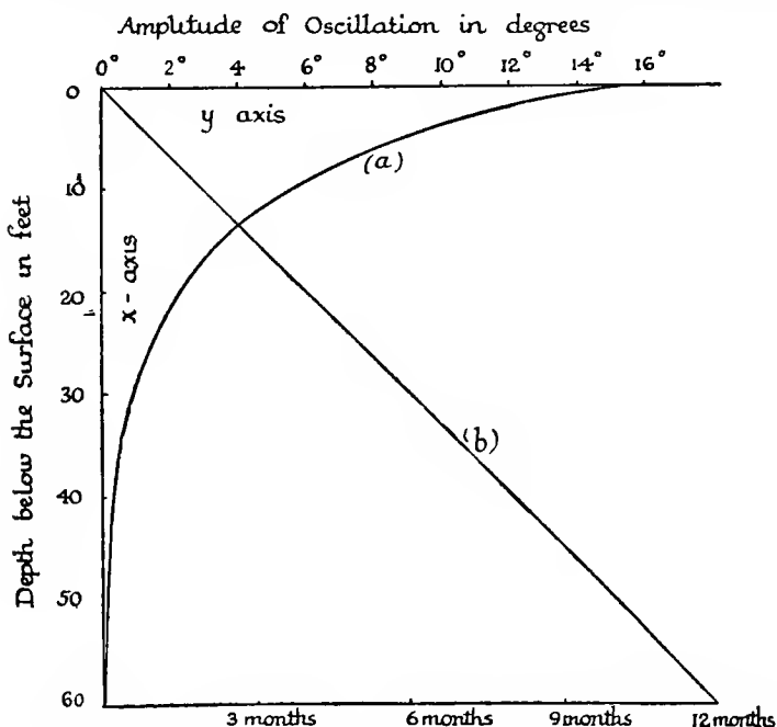
Fig. 26.—a, Curve showing Amplitude of Temperature Oscillations at different depths. b, Line showing Lag of Maximum Temperature with depth.
