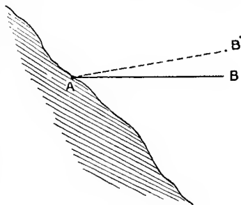
Fig. 52.—Heating Effect in a Valley
