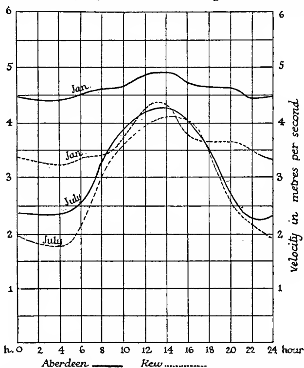
Fig. 41.—Diurnal Variation in Wind Velocity for January and July for the period 1881-1910
