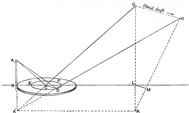
Fig. 59.—Illustrating the Theory of the Fineman Nephoscope
