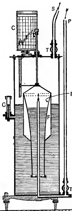
Fig. 36.—Section Diagram of Recording Apparatus of Dines' Pressure-tube Anemometer
