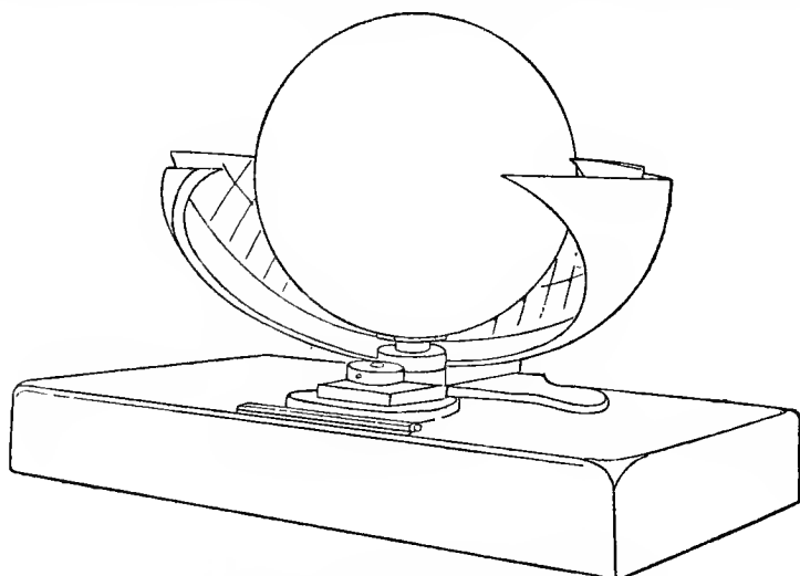
Fig. 60.—The Campbell-Stokes Sunshine Recorder
