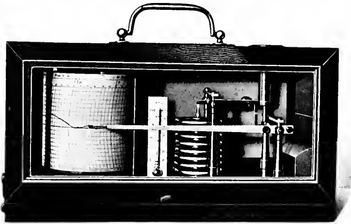
Fig. 30.—Barograph, M.O. pattern
