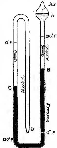
Fig. 17.—The Principles of Six's Thermometer
