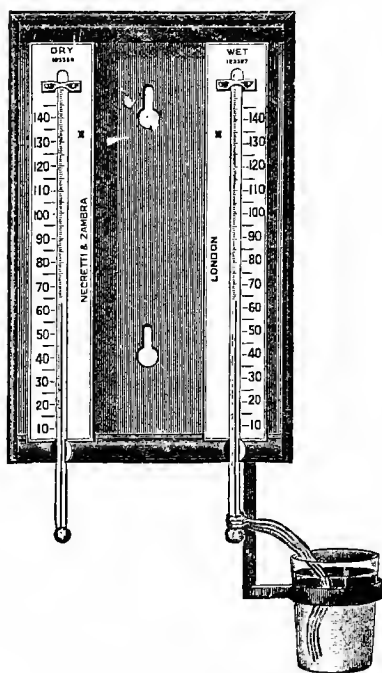
Fig. 54.—Wet- and Dry-bulb Hygrometer
