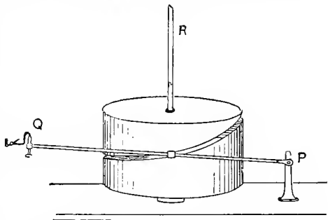
Fig. 37.—Principle of the Munro-Rooker Direction Recorder
