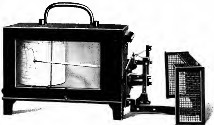
Fig. 53.—Hair Hygograph, M.O. pattern, with guard removed to show bundle of hairs and lever
