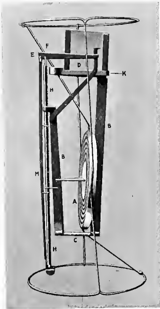
Fig. 80.—Meteorograph: general view
