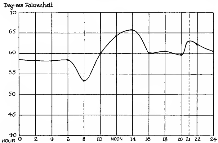
Fig. 2.—Temperature Variation at Aberdeen on 1st August, 1919
