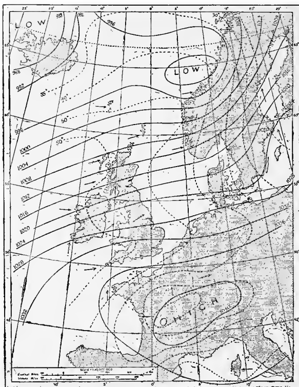
Fig. 103a.—South-westerly type, showing pressure and temperature distributions. Pressure expressed in millibars, temperature in degrees F. (7 h. chart, 16th January, 1920.)
