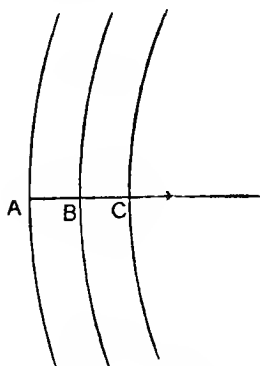
Fig. 44.—Pressure Gradient
