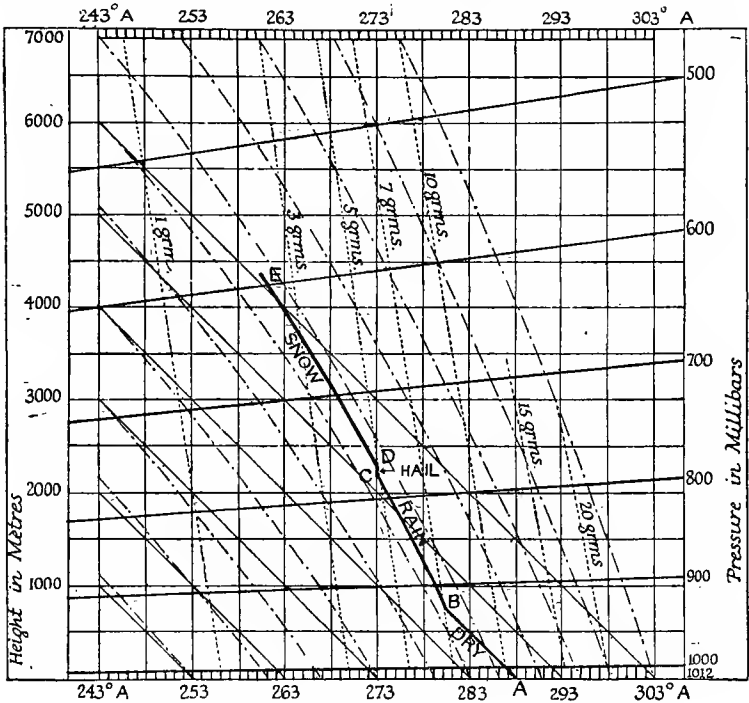
Fig. 58.—Adiabatic Diagram (modified from Neuhoff-Hertz)
