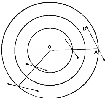
Fig. 47.—Cyclonic System
