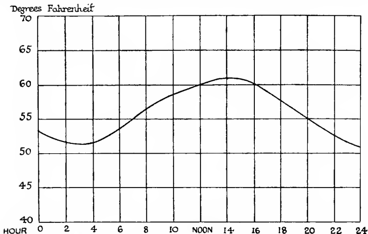
Fig. 1.—Temperature Variation at Aberdeen on 3rd August, 1919
