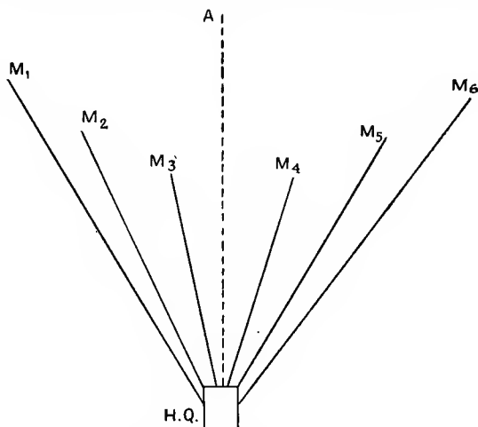
Fig. 99.—Arrangement of Microphones in Sound-ranging
