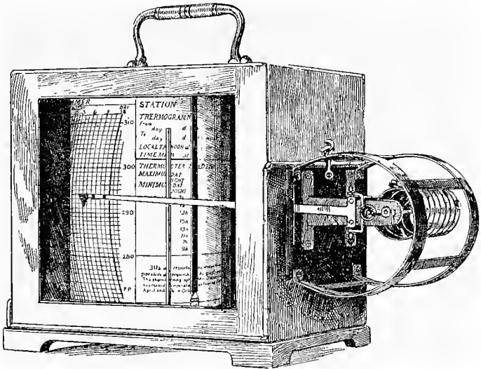
Fig. 19.—Thermograph
