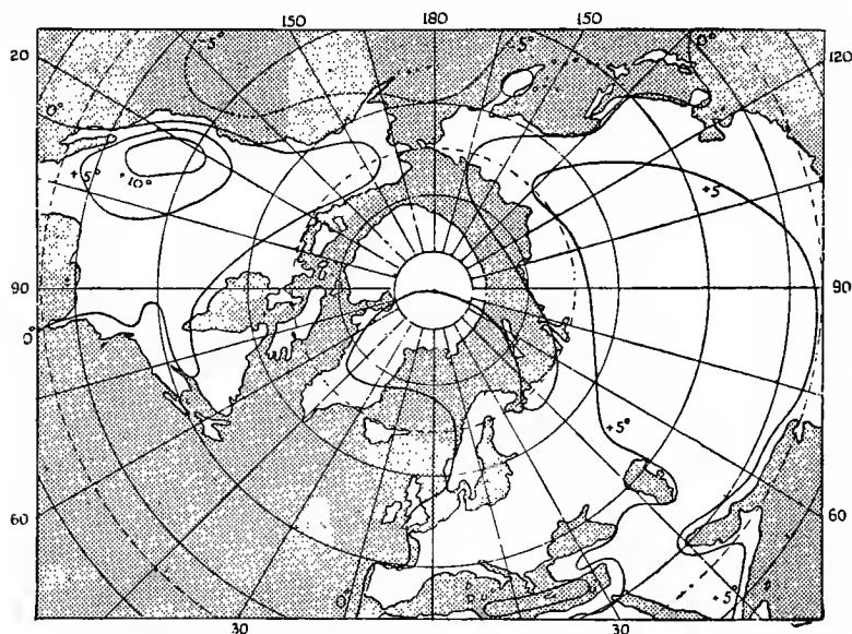
Fig. 25. —Isanomalies of Temperature for July in Degrees Absolute (after Angot)
