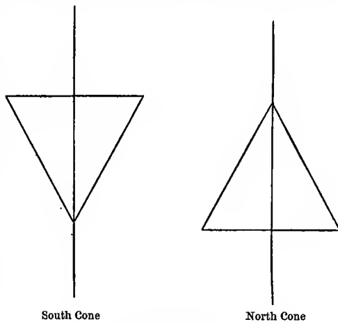
Fig. 100.—Storm Signals
