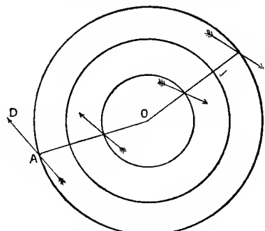
Fig. 48.—Anticyclonic System
