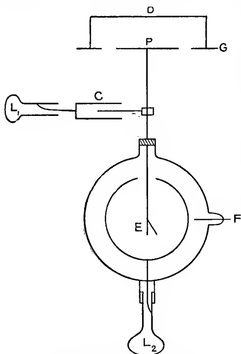
Fig. 92.—Diagram of Wilson's Apparatus (original arrangement)
