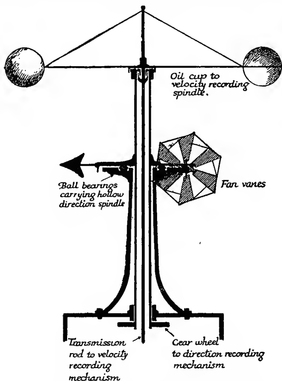
Fig. 38.—Sectional View of Robinson-Beckley Self-recording Cup Anemometer
