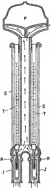
Fig. 13.—Assmann's Ventilation Thermometer
