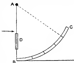
Fig. 34.—Showing Principle of Swinging-plate Anemometer
