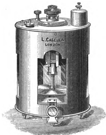
FIG. 67.—Thomson's Portable Electrometer.
