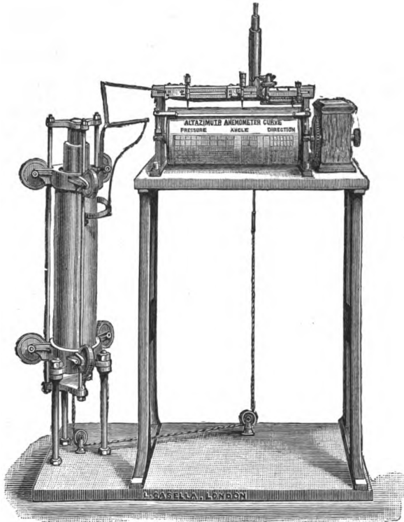
FIG. 61B.—Casella's Altazimuth Anemometer.
