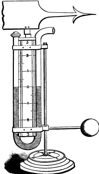
FIG. 57.—Lind's Anemometer.
