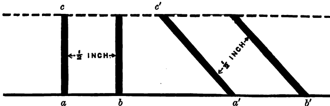
FIG. 68.—Diagram illustrating the effect of the perpendicular and the oblique falling of the Sun's rays.
