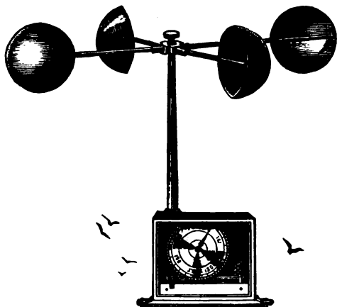
FIG. 58.—Robinson's Anemometer.
