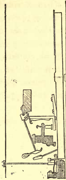
6. John Brinsmead's Check Repeater action.
