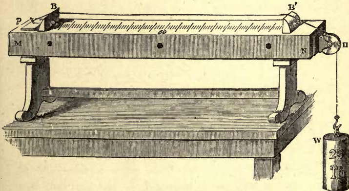
THE MONOCHORD.
