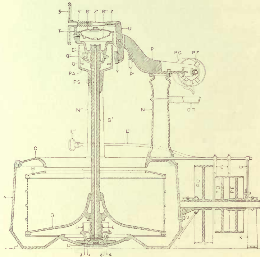
Parts Lettered for Convenience in Ordering Repairs
