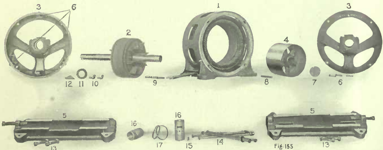
Displayed View of 40 H. P. Squirrel Cage Induction Motor.
