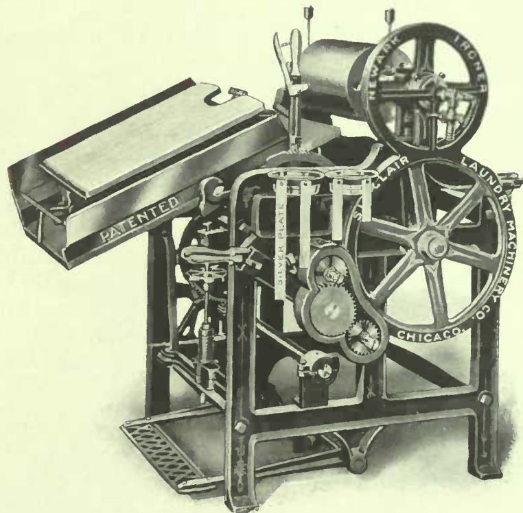
Bosom Ironer. No. 478.
