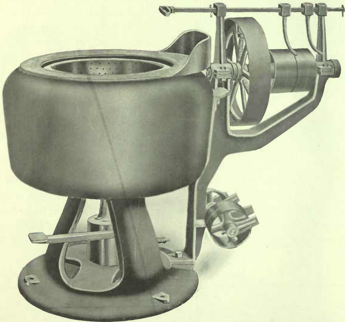
26 Inch Countershaft Attached. No. 173
