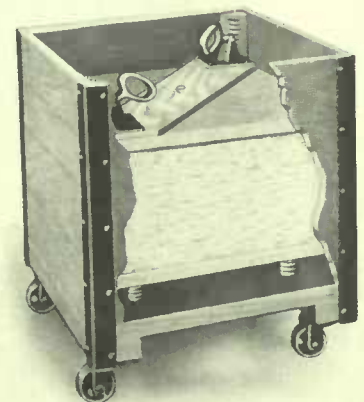
Showing Springs Under Follow Up Bottom
