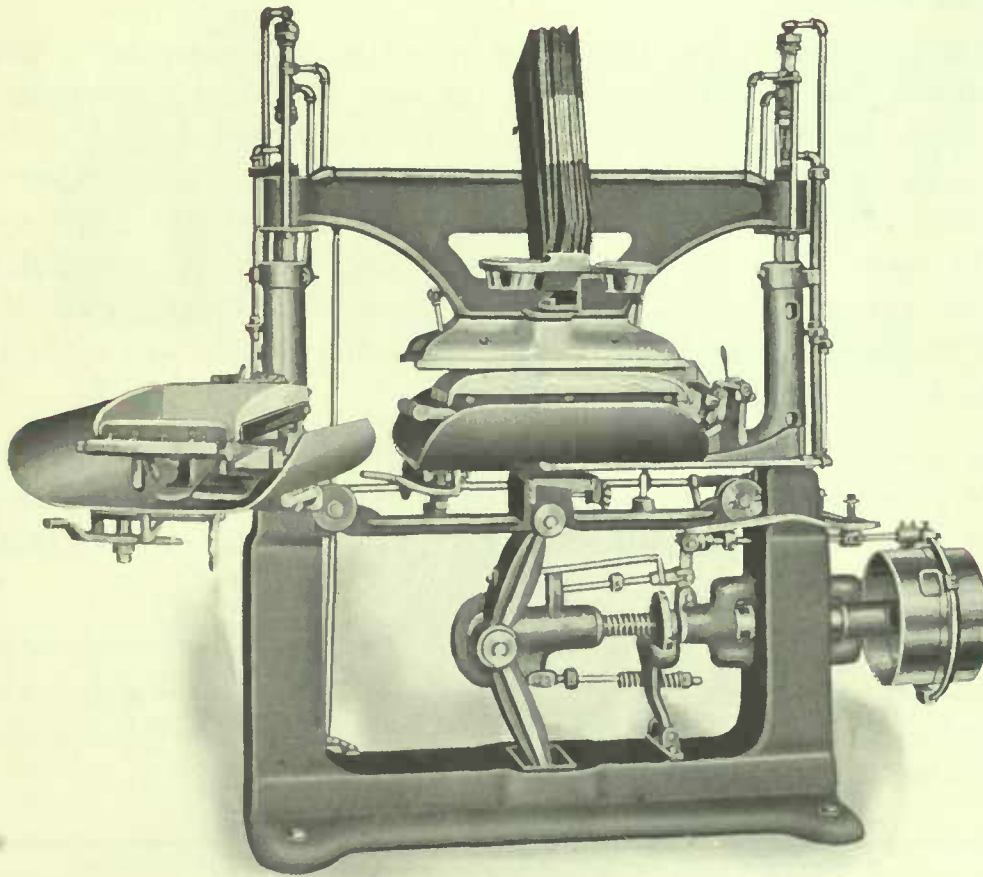
Toronto Bosom Press.
