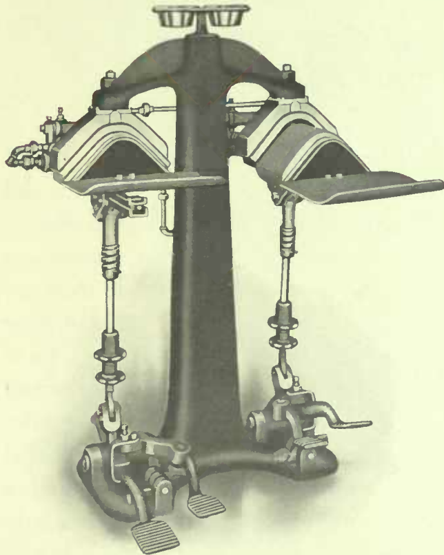
Double Saddle Cuff Press. No. 393.
