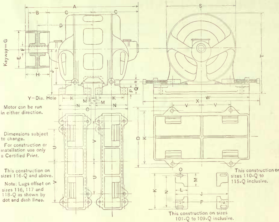
Dimensions Form "Q" Machines, 60 Cycles.
