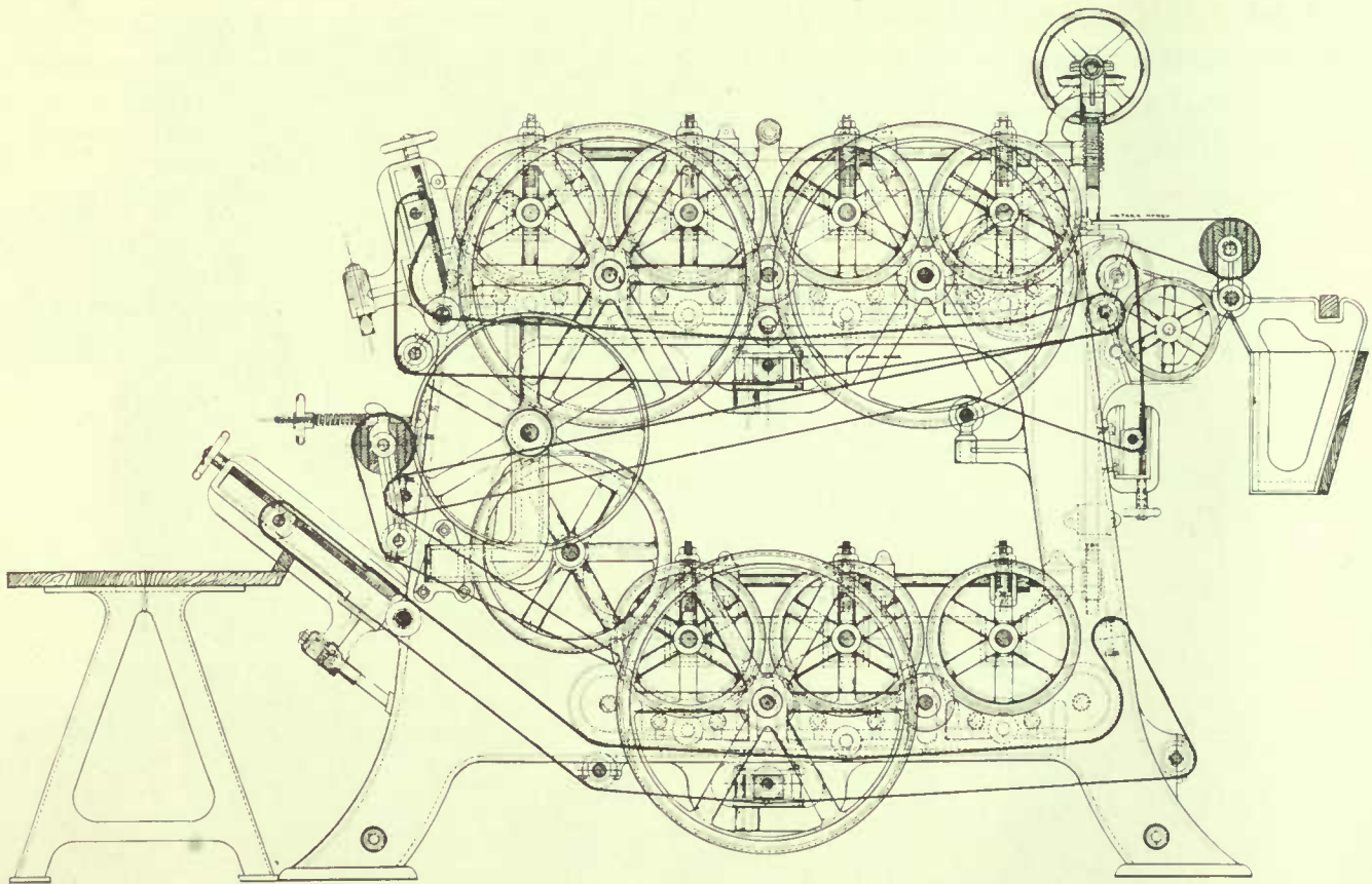
END ELEVATION SHOWING ARRANGEMENT OF ROLLS, CHESTS AND APRONS
