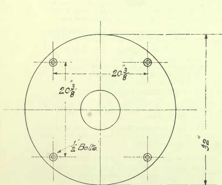
PLAN OF BOLT HOLES FOR 20" TORONTO IMPROVED EXTRACTOR.
