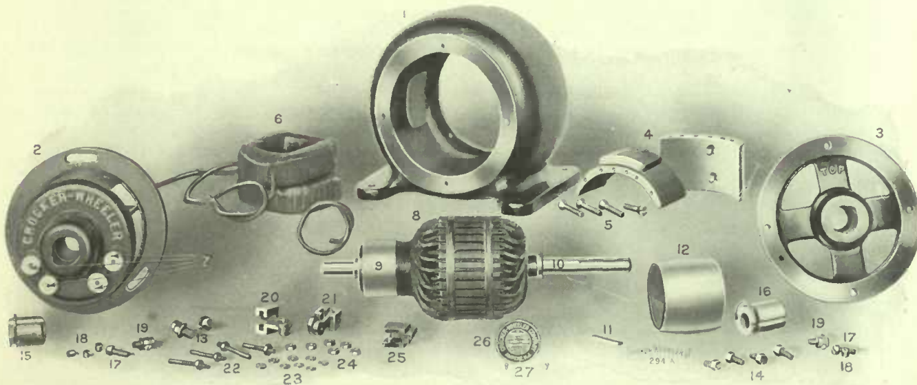
Form L Motors
