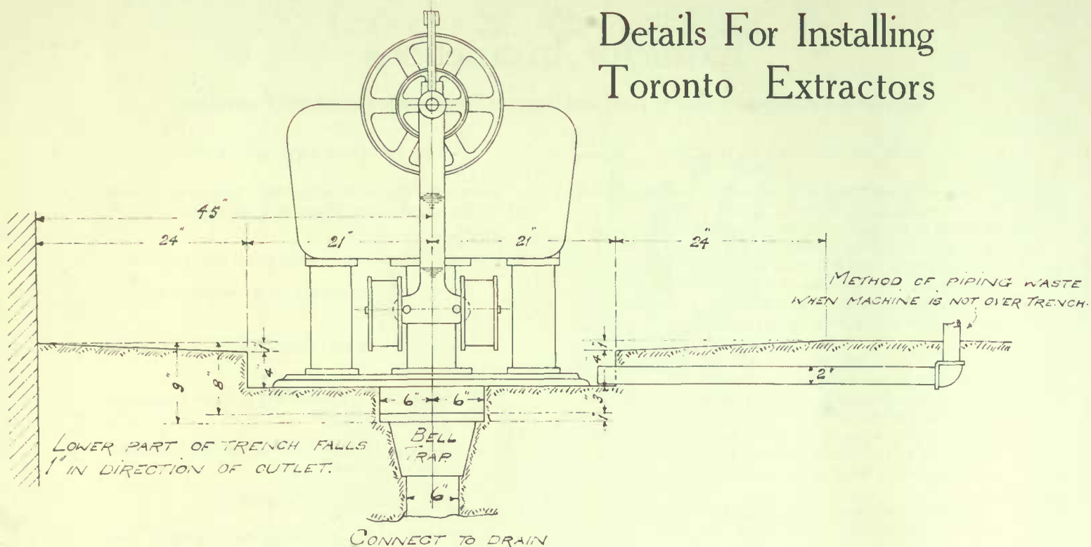
Details of Trench, Showing Extractor Located
