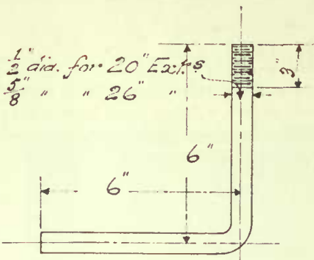
FOUNDATION BOLTS. TOP OF BOLT TO EXTEND 3" ABOVE FINISHED FLOOR LEVEL.
