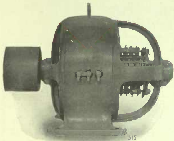
Form I Machine
