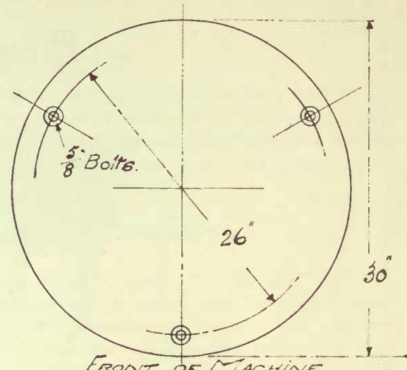
FRONT OF MACHINE. PLAN OF BOLT HOLES FOR 26" TORONTO SOLID CURB EXTRACTOR.
