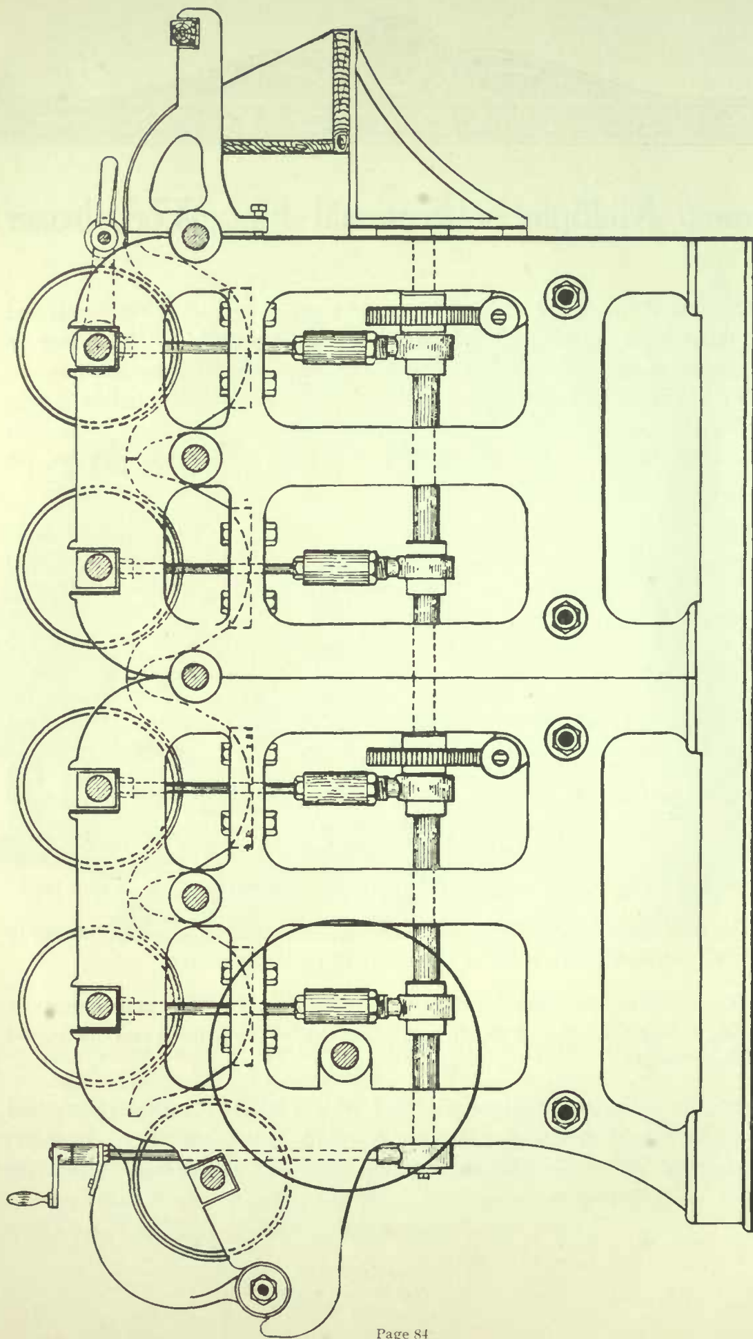
Sectional View, Five Roll Multiple Flat Work Ironer
