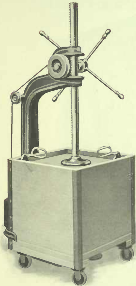
Showing Truck in Position for Applying Pressure
