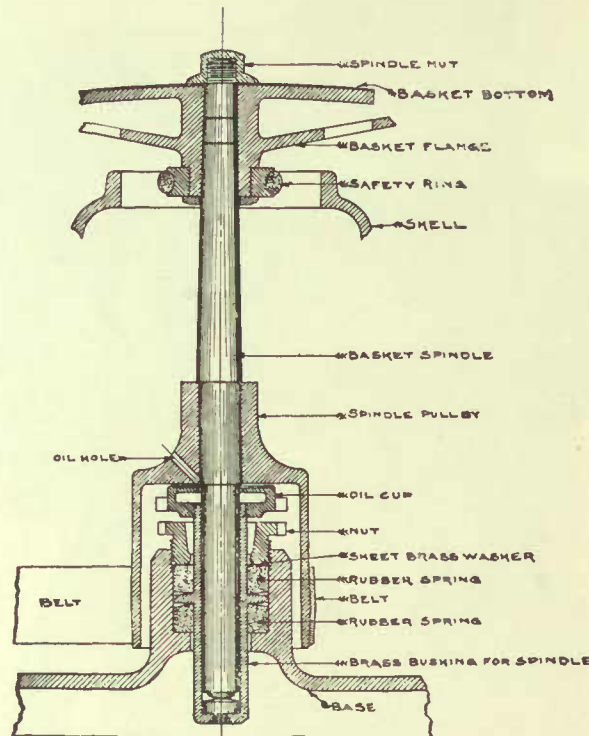
Sectional View through Spindle
