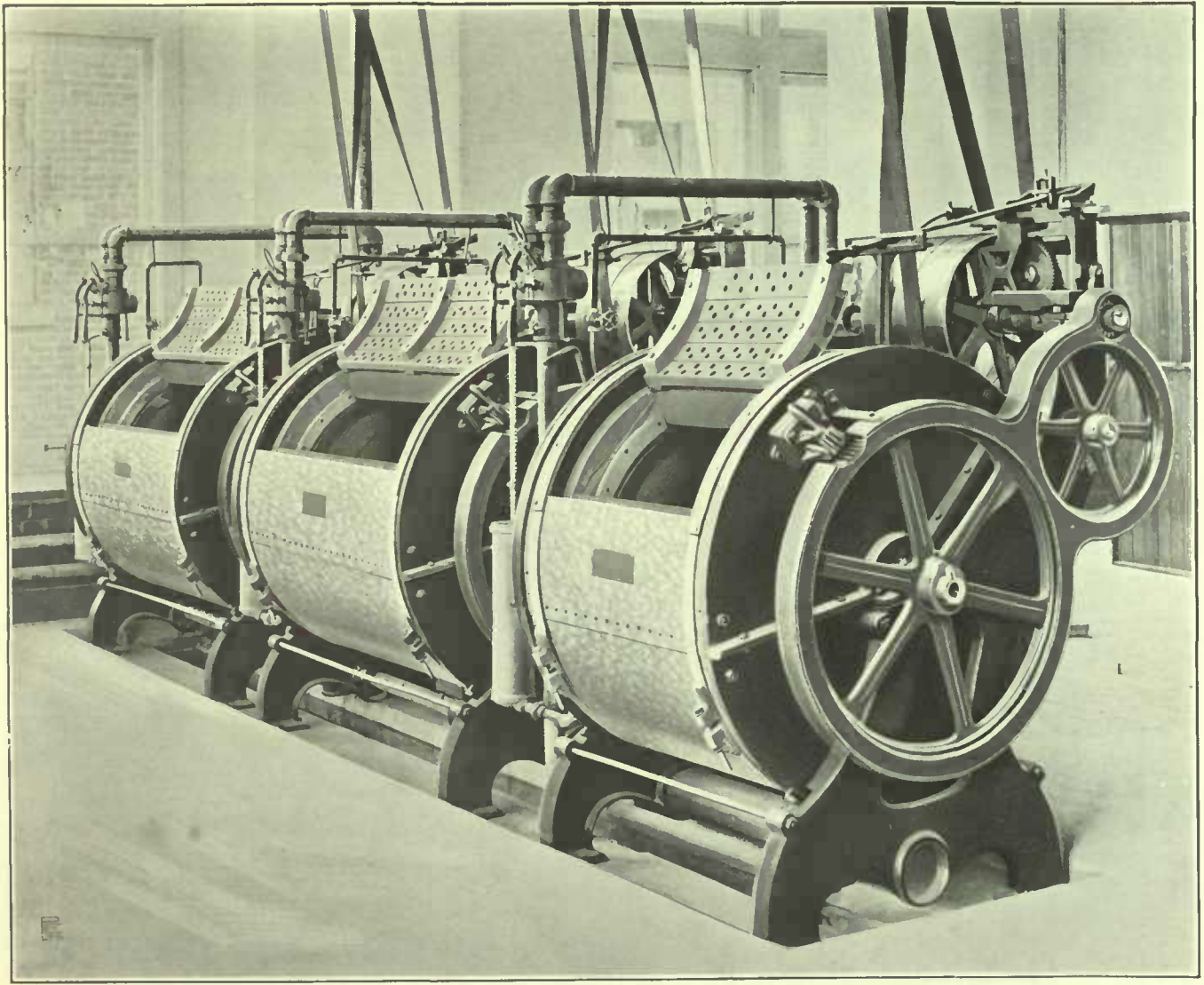
An ideal installation of three FAMOUS FORTY Elevated Movement Washers in the New Method Laundry, Toronto, equipped with the Yates Automatic Washer Inlet Valves.
