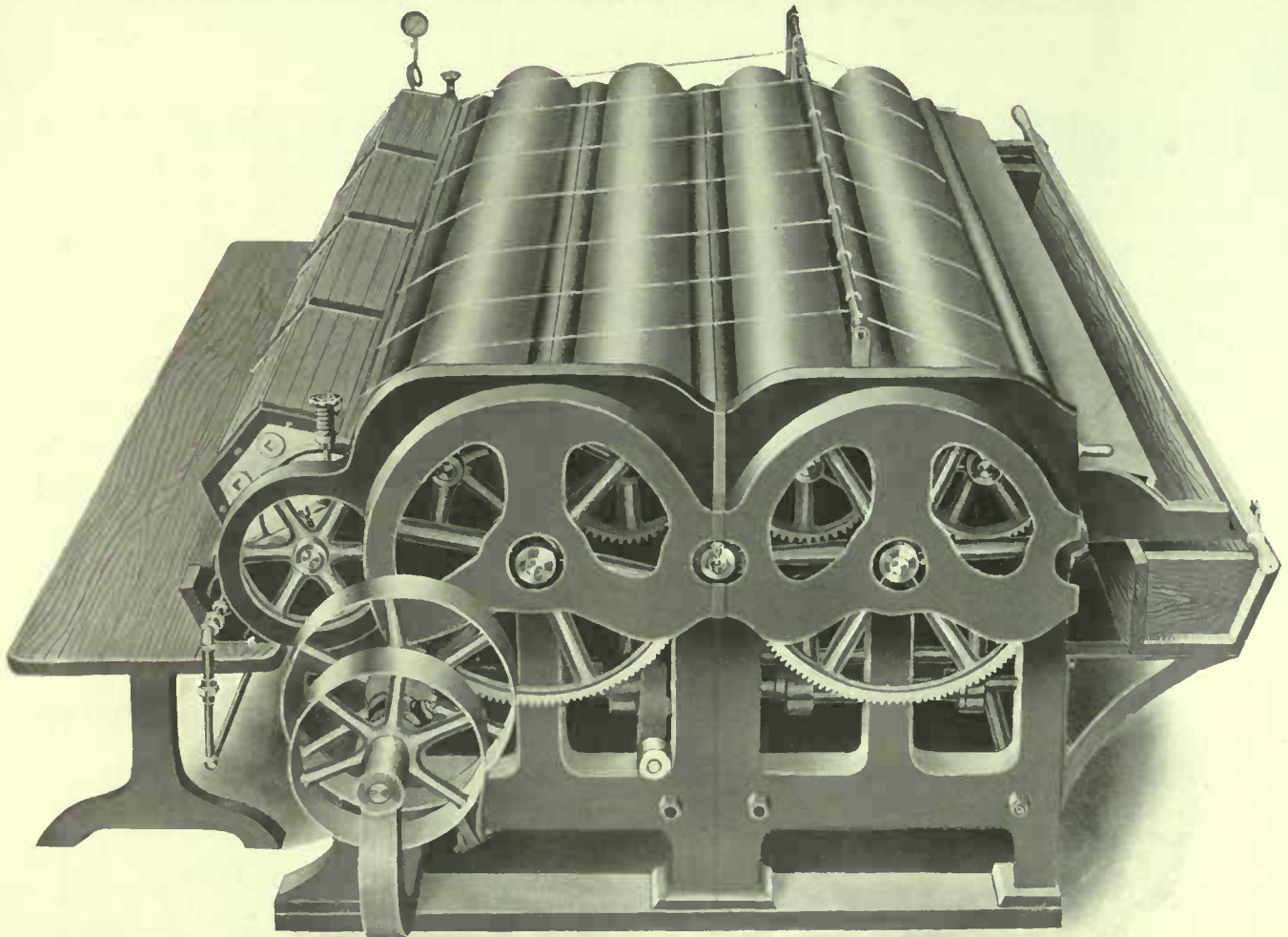
Five Roll, 120 inch Multiple Flat Work Ironer
