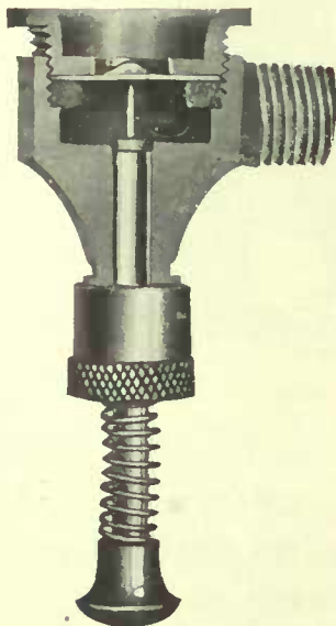
Fig. 255 Sectional View DuSpray Nozzle
