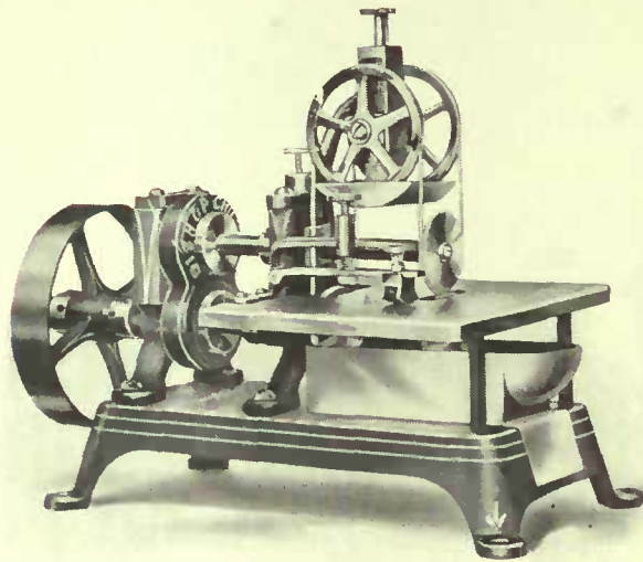
Cord Seam Dampeners. No. 317.
