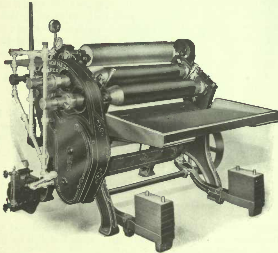
Showing Steam Heated Ironer No. 305.
