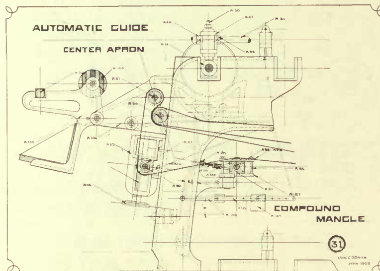
Automatic Apron Guide—Centre or Intermediate Apron
