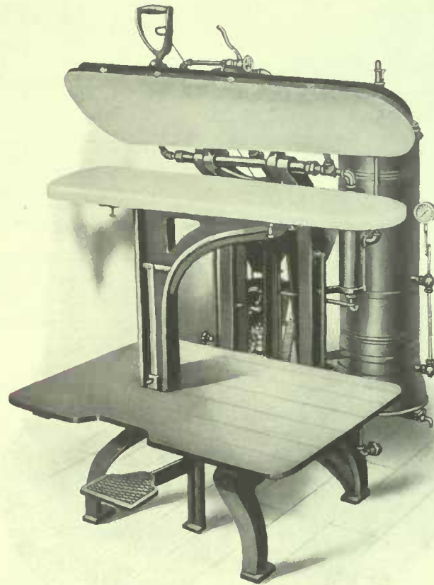
Front View. Shown With Boiler Attached.
