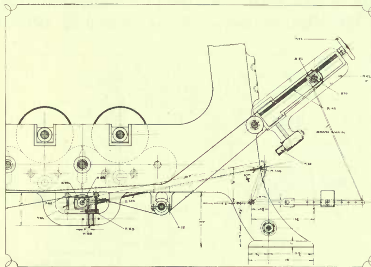
Automatic Apron Guide—Lower Apron
