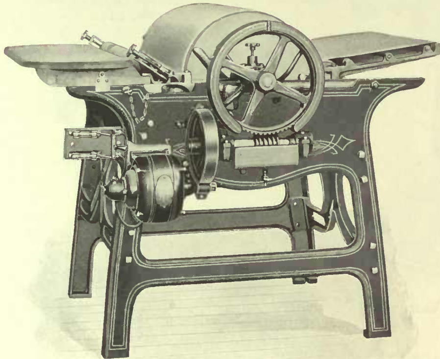
24 inch Collar Starcher, with Motor Attached. Motor, 1/8 H. P.
