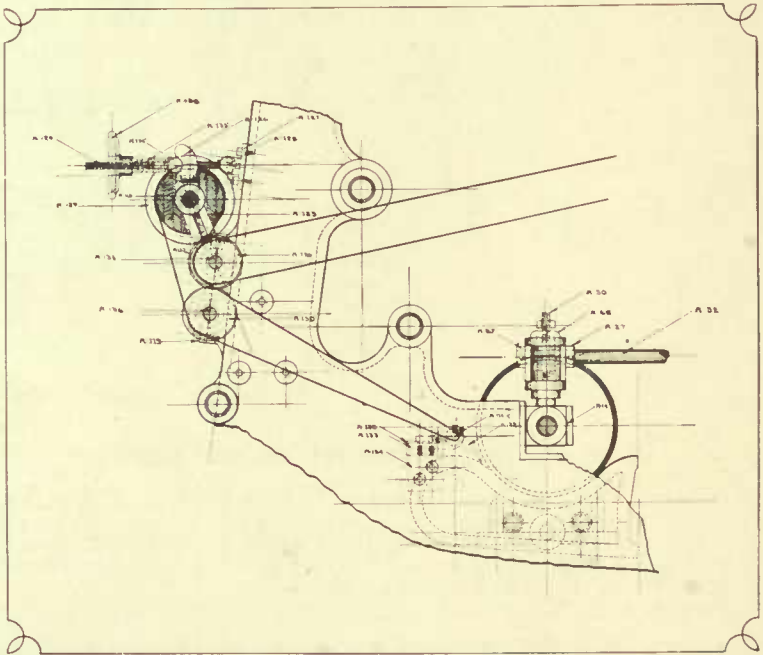
Lower Ribbon Apron Feed
