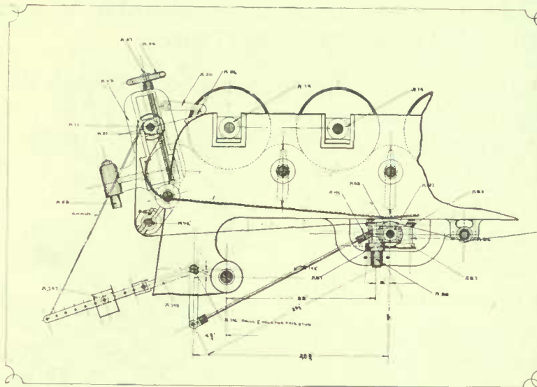
Automatic Apron Guide—Upper Apron
