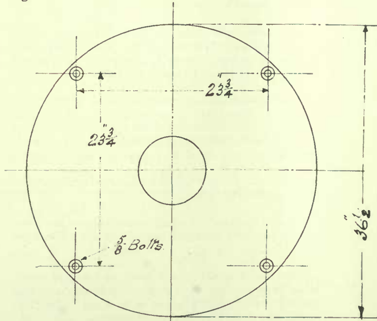
PLAN OF BOLT HOLES FOR 26" TORONTO IMPROVED EXTRACTOR.
