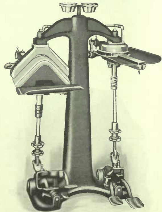
Combined Yoke and Neckband Press. No. 394.
