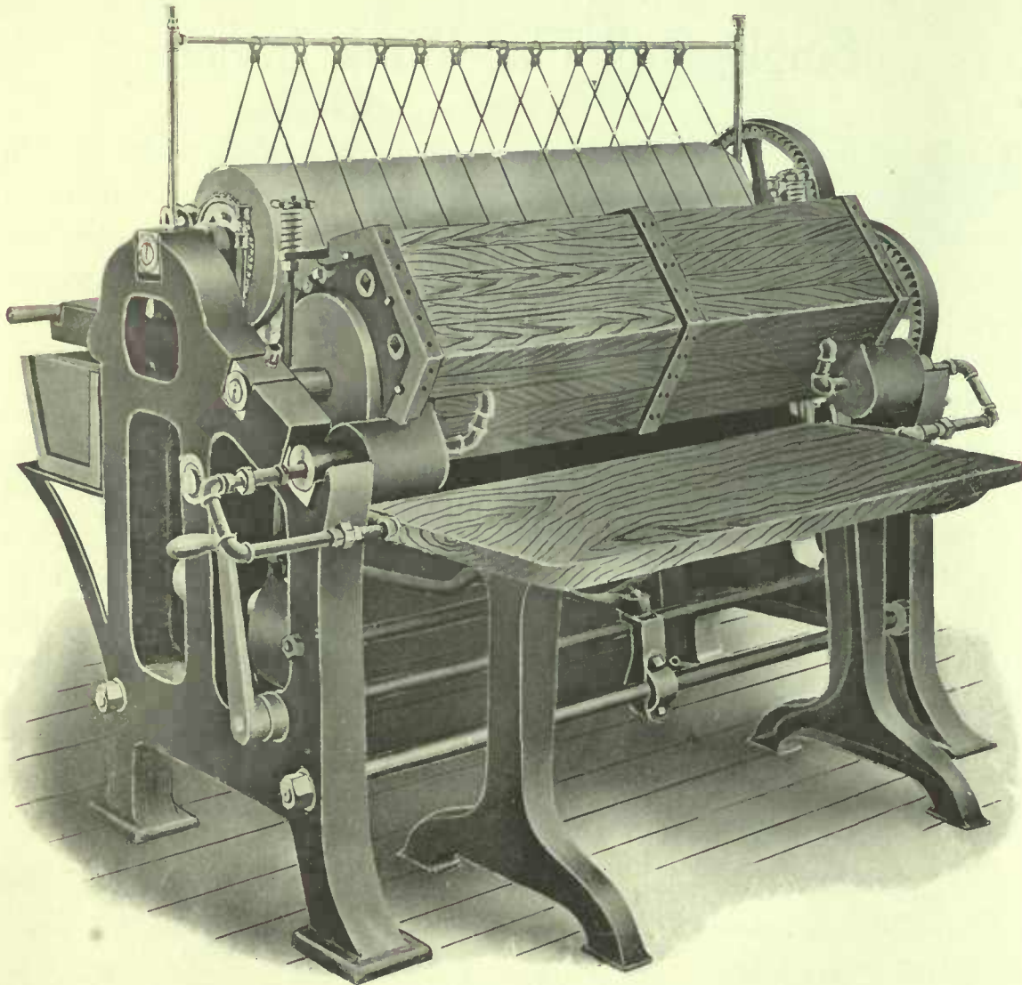
Delivery Side of 48 inch Machine.
