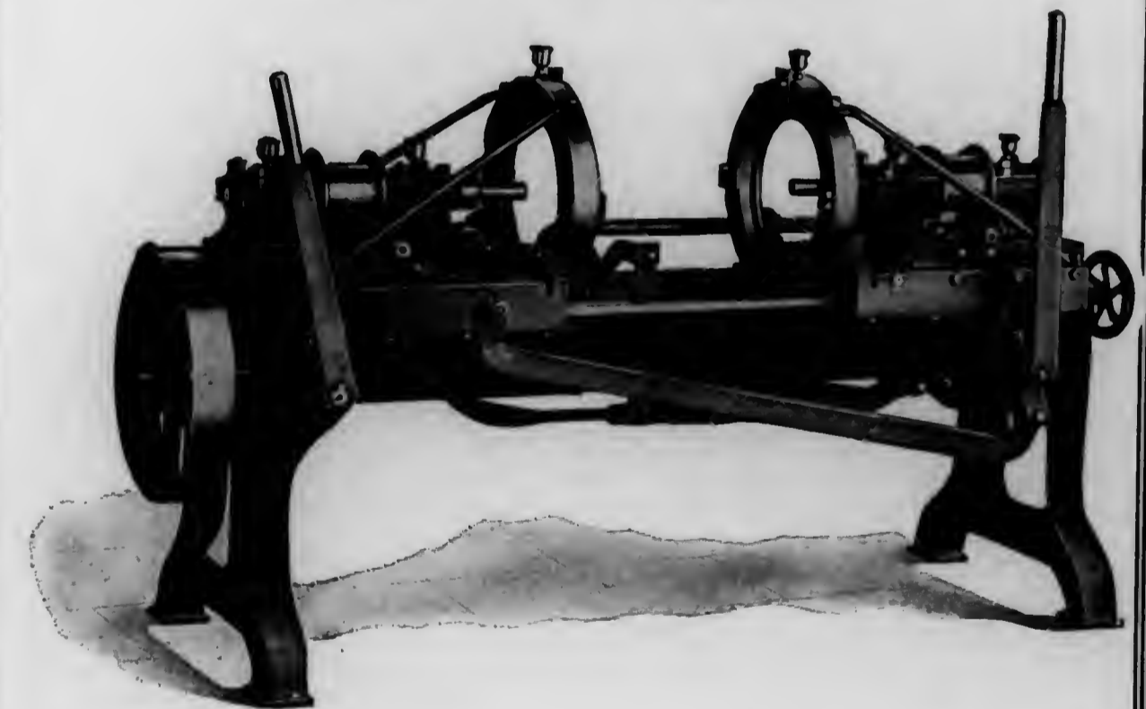
KEG CROZER—4-inch Diameter Head to 11-inch Diameter Head and Up to 20-inch Long Staves
