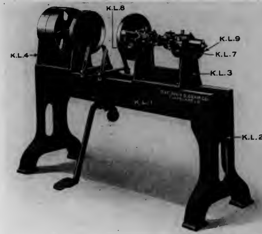
KEG LATHE Also Can Fit Up With Plane and Rod and Rest
