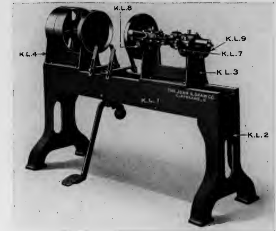
KEG LATHE Also Can Fit Up With Plane and Rod and Rest
