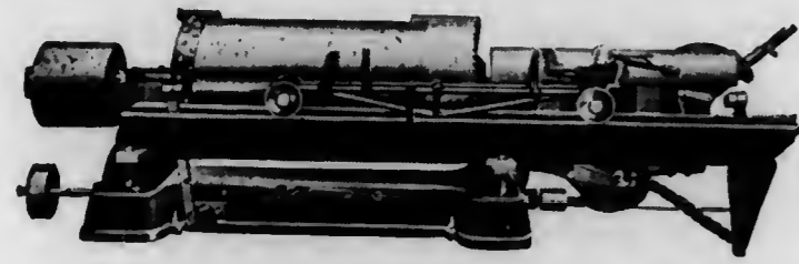
26" x 53" SPECIAL STAFF SAWING MACHINE SAWS STAVES ON 26" CIRCLE FROM 20" TO 42" LONG
