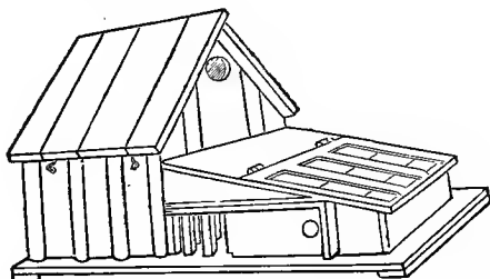
HEN AND CHICKENS' COOP. (Described on page 110.)
