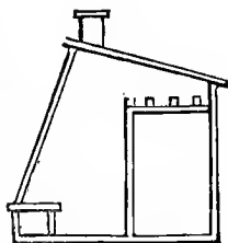
FIG. 2 — A CROSS SECTION.
