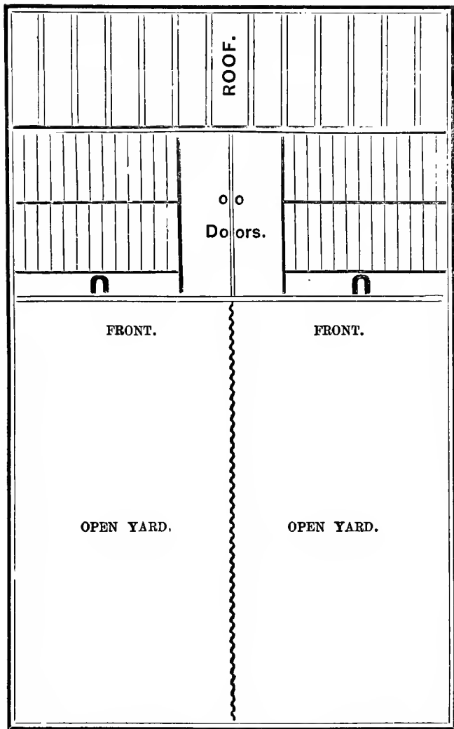
A CHEAP, DOUBLE BATTENED-ROOF SUMMER FOWL-HOUSE.
