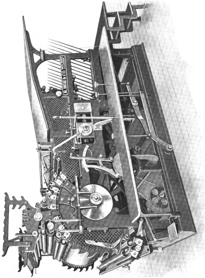
ROTARY ZINCOGRAPHIC OR ALUMINUM PRESS
