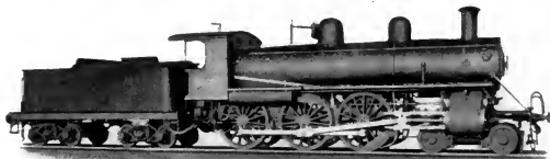
BALANCED COMPOUND TEN-WHEELED LOCOMOTIVE For the Italian Government Railways
