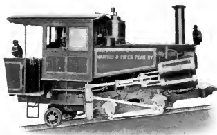
RACK LOCOMOTIVE, ABT SYSTEM
