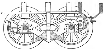
BALDWIN FLEXIBLE BEAM TRUCK, 1842—ELEVATION
