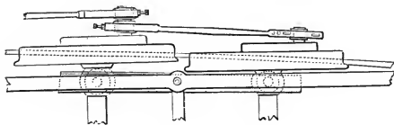
BALDWIN FLEXIBLE BEAM TRUCK, 1842—HALF PLAN
