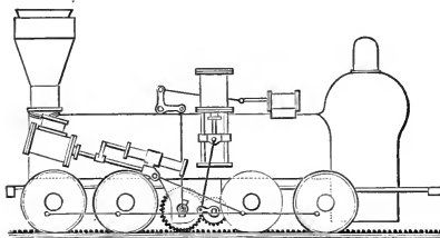
BALDWIN ENGINE FOR RACK RAIL, 1847
