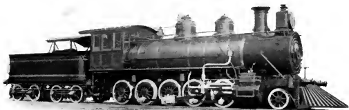
DECAPOD LOCOMOTIVE
