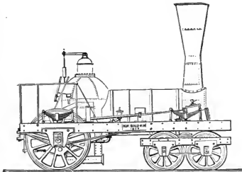
BALDWIN LOCOMOTIVE, 1834
