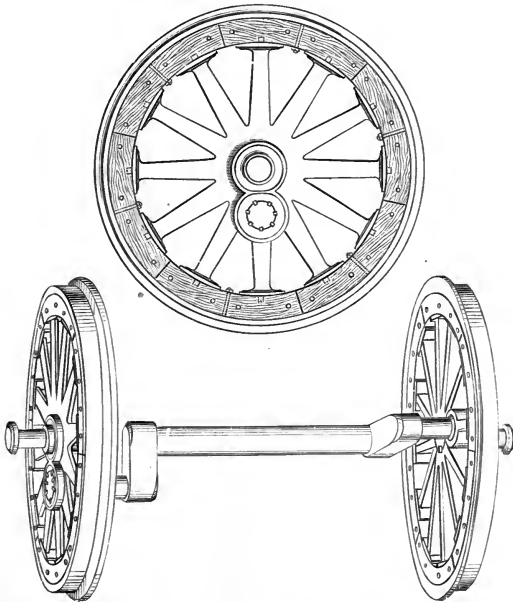
BALDWIN COMPOUND WOOD AND IRON WHEELS, 1834
