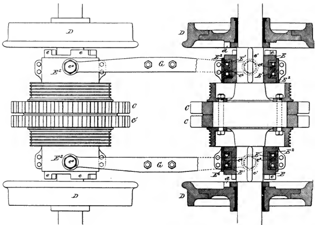
CLUTCH USED ON LOCOMOTIVE FOR PEÑOLES MINING CO.
