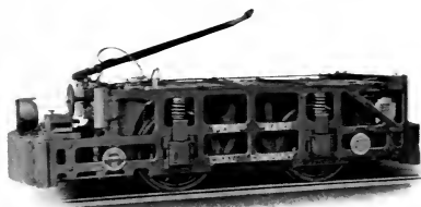
ELECTRIC MINING LOCOMOTIVE With Cast Steel Bar Frames
