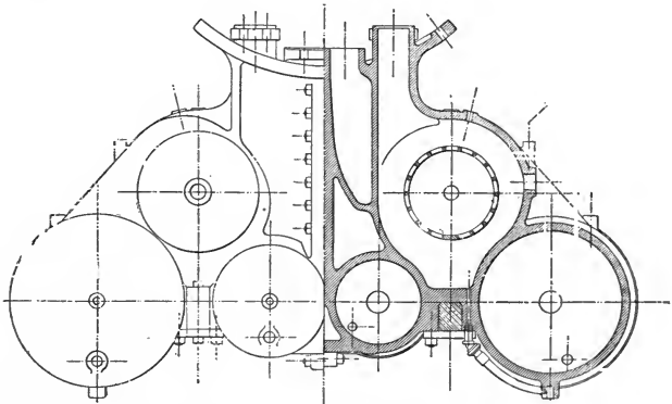
CROSS SECTION OF BALANCED COMPOUND CYLINDERS
