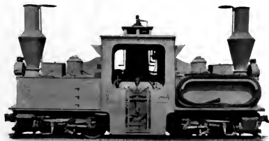
PECHOT TYPE LOCOMOTIVE For the French Government
