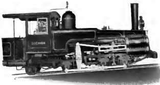
COMBINATION RACK AND ADHESION LOCOMOTIVE For the Peñoles Mining Co.
