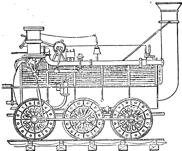
FIG. 13.—THE FIRST SUCCESSFUL LOCOMOTIVE. HACKWORTH'S "ROYAL GEORGE," STOCKTON AND DARLINGTON RAILWAY, 1827
