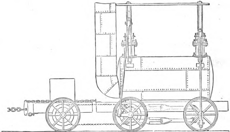
FIG. 7.—STEPHENSON AND DODD'S PATENT ENGINE, BUILT IN 1815
