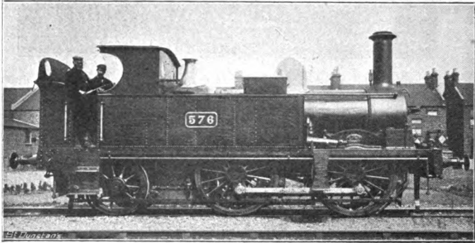
FIG. 135.— 4-COUPLED-IN-FRONT PASSENGER TANK ENGINE, G.W.R.
