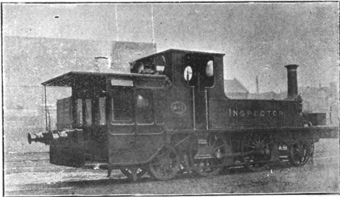
FIG. 105.—"INSPECTOR," LONDON, BRIGHTON, AND SOUTH COAST RY.
