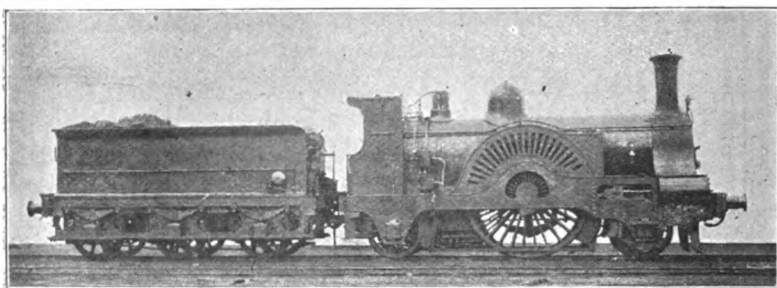
FIG. 85.—CONNER'S 8FT. 2IN. "SINGLE" ENGINE, CALEDONIAN RAILWAY (REBUILT)
