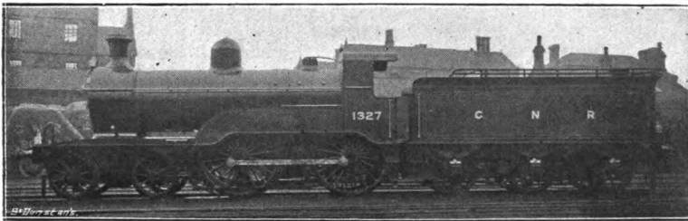
FIG. 137.— THE LATEST TYPE OF 6FT. 6IN. COUPLED ENGINE, GREAT NORTHERN RAILWAY
