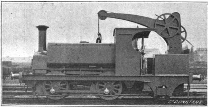
FIG. 89.—LOCOMOTIVE AND TRAVELLING CRANE, N.L.R.
