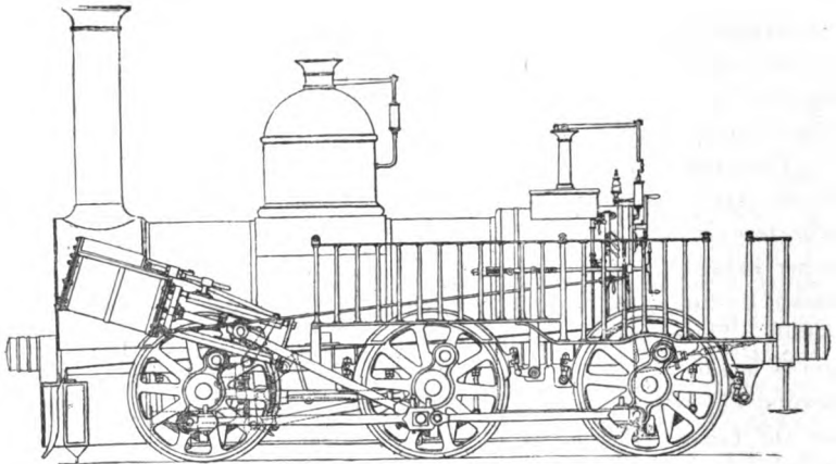
FIG. 34A.— PATON AND MILLAR'S TANK ENGINE FOR WORKING ON THE COWLAIRS INCLINE, GLASGOW
