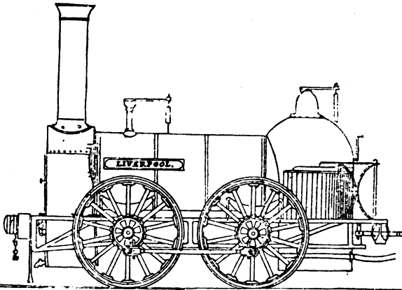
FIG. 17.—BURY'S ORIGINAL "LIVERPOOL," THE FIRST ENGINE WITH INSIDE CYLINDERS AND CRANKED DRIVING AXLE. COUPLED WHEELS, 6ft. DIAMETER.
