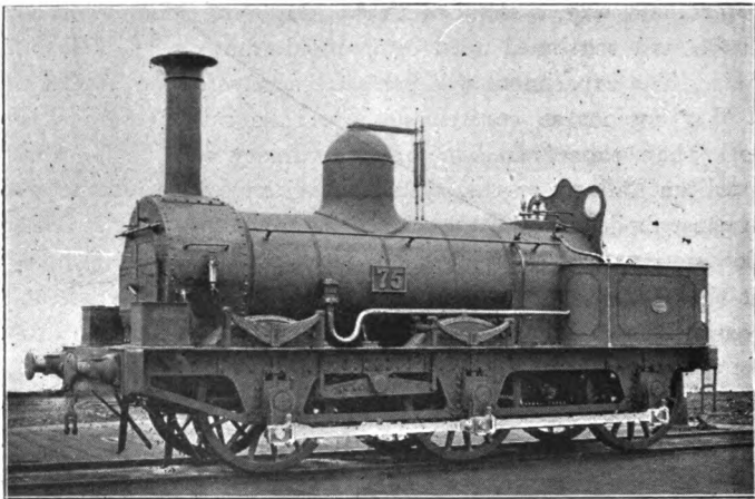
FIG. 81.—SIX-COUPLED MINERAL ENGINE, TAFF VALE RWY., BUILT 1860
