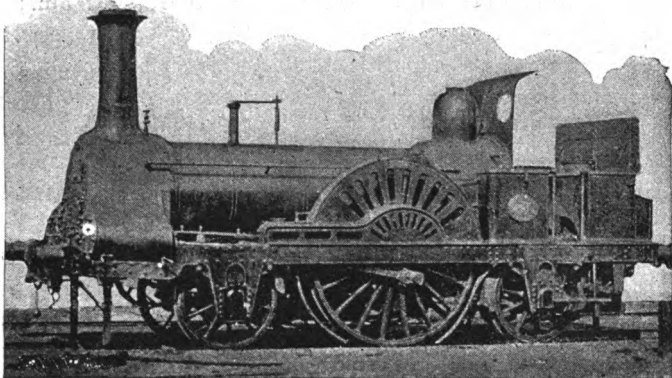
FIG. 62.—ONE OF J. V. GOOCH'S "SINGLE" TANK ENGINES, EASTERN COUNTIES RAILWAY
