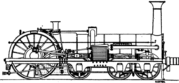
FIG. 55.—CRAMPTON'S "LIVERPOOL," L. AND N.W.R.
