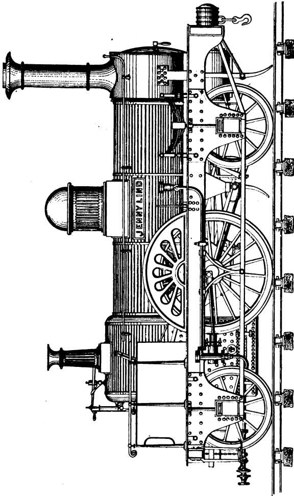
Fig. 59.—E. B. Wilson's Standard Pattern, 1849.
