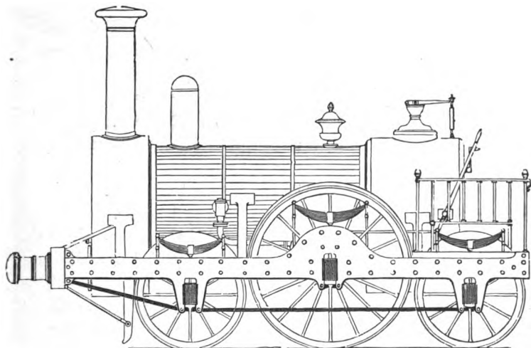
Fig. 45.—Grand Junction Railway, 1838.
