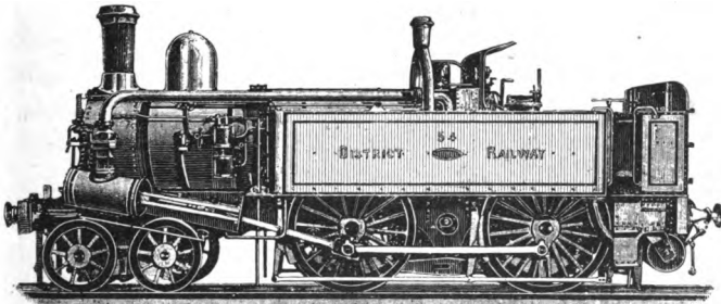
Fig. 83.—Metropolitan District Engine.
