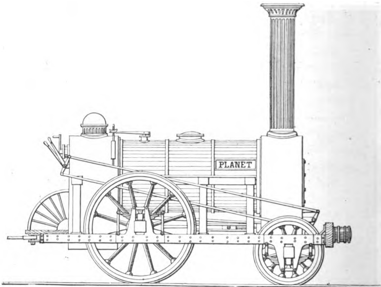
Fig. 20.—“Planet,” No. 9, Liverpool and Manchester Railway, 1830.
