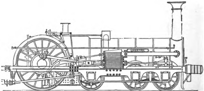
Fig. 58.—"Liverpool," London and North-Western Railway, 1848.
