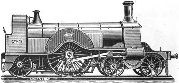
Fig. 78.—Type of Great Northern Express Engine, 1870 to 1887.
