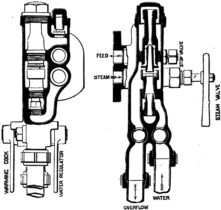
Fig. 92.—Details of Injector.
