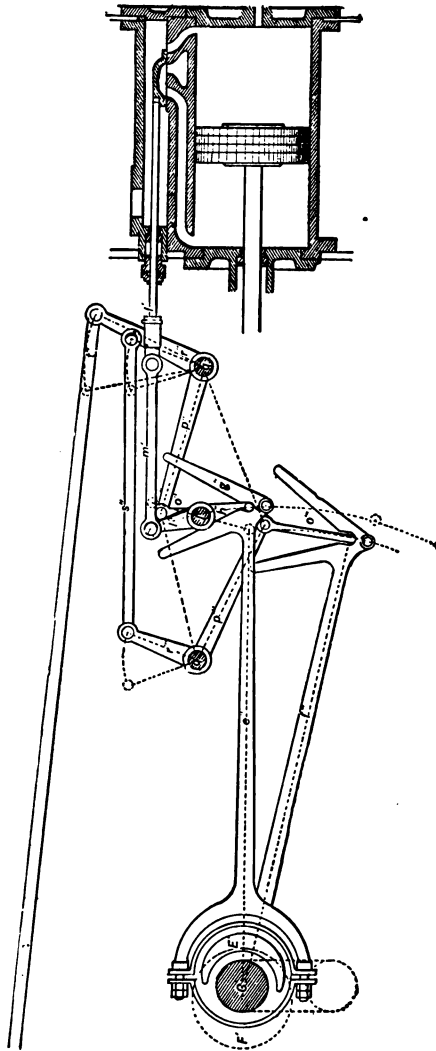
Fig. 51.—Stephenson's Fork Motion, 1835 to 1842.
