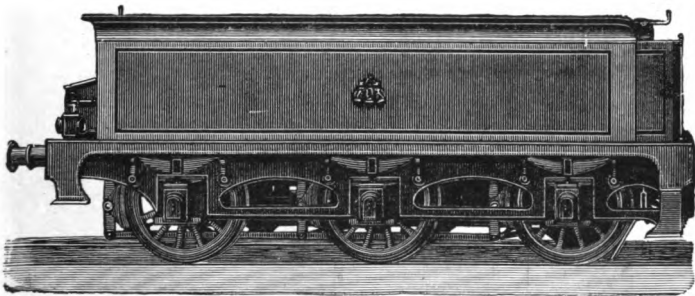
Fig. 77.—Caledonian Tender, No. 123.
