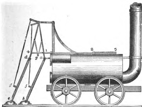
Fig. 4.—"Brunton's Engine," 1813.
