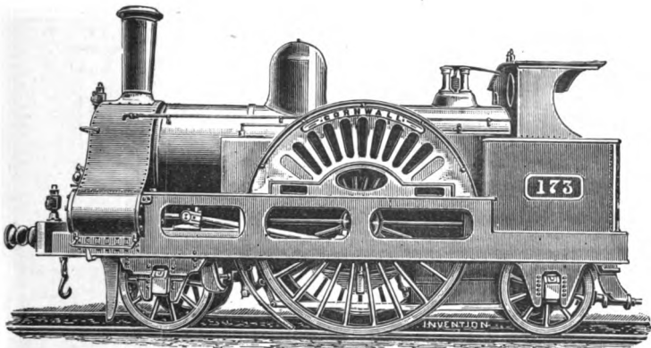
Fig. 57.—"Cornwall," London and North-Western Railway, 1863 to 1893.
