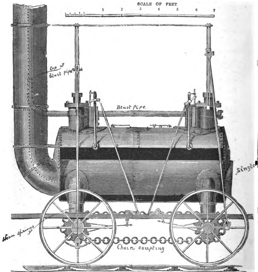
Fig. 6.—George Stephenson's Killingworth Engine, 1816.
