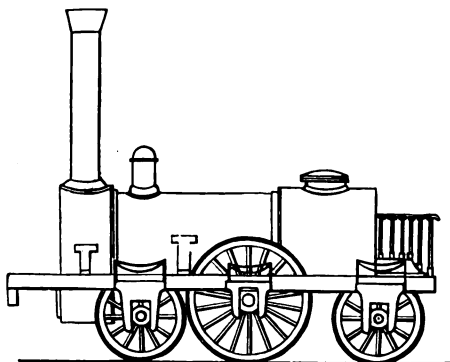
Fig. 34.—"Patentee," No. 33, Liverpool and Manchester Railway, January, 1834.
