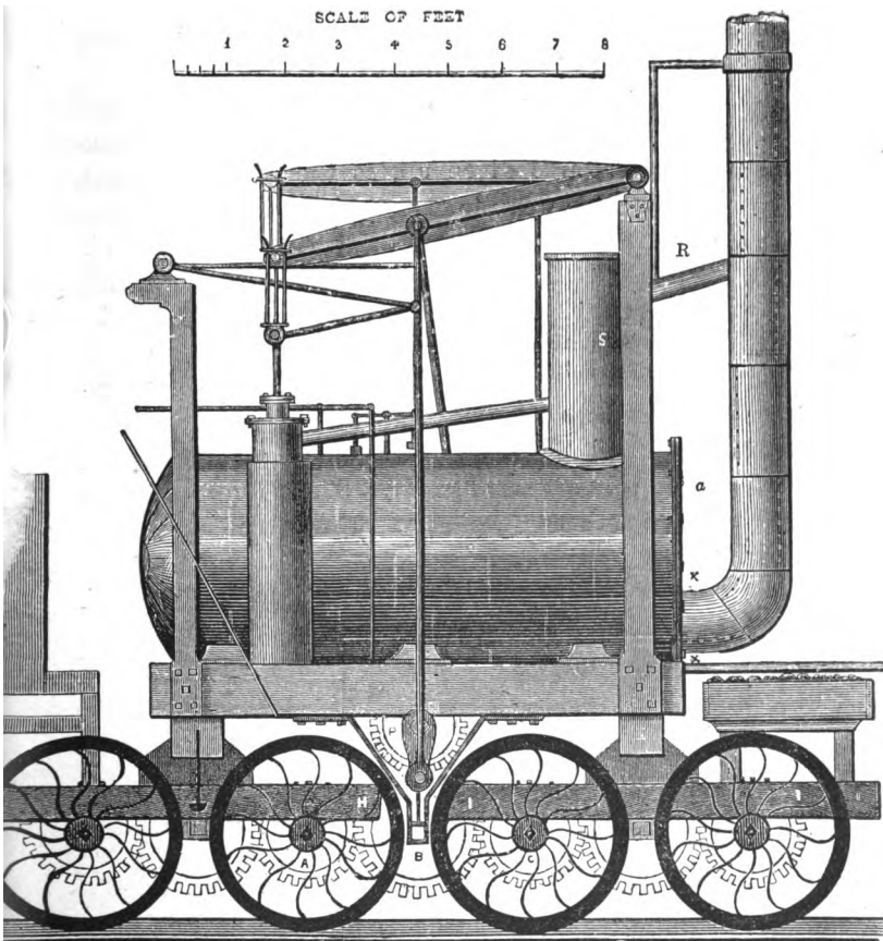
Fig. 8.—“Puffing Billy,” as rebuilt 1815.
