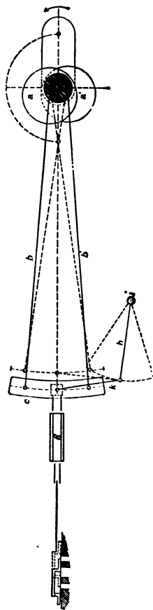
Fig. 52.—Howe's Link Motion, 1842.
