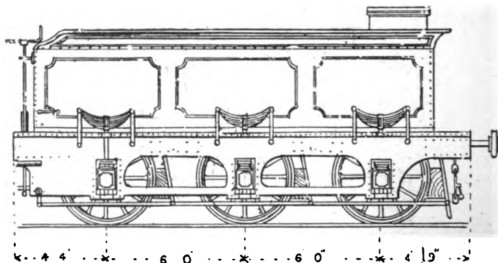
Fig. 67.—Midland Tender, 1870.
