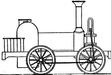
Fig. 27.—"Caledonian," No. 28, Liverpool and Manchester Railway, 1832.
