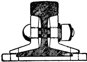
Chicago & North-Western Railway Standard 60-lb. Rail, A. D. 1897.
