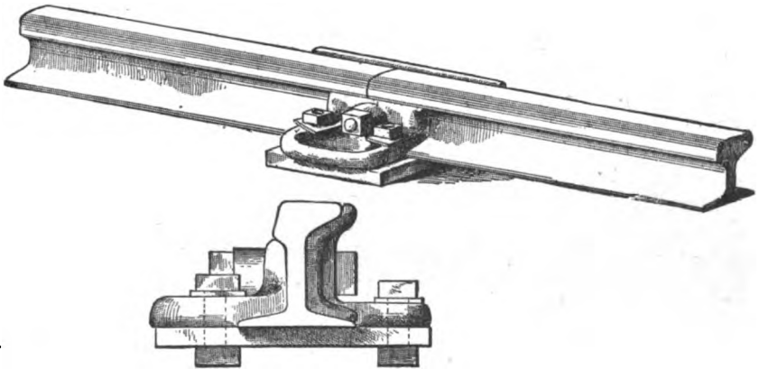
Joint Fixture used on Western railroads, A. D. 1860.
