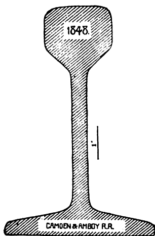
92-pound Rail, 7 inches high.
