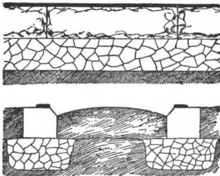
Stone Stringer and Strap Rail, Baltimore & Ohio Railroad, A. D., 1823. This was a favorite American device.
