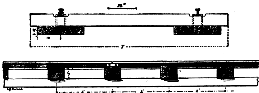
Stevens Rail, Vicksburg & Jackson Railroad, A. D. 1841.
