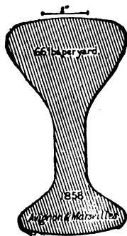
Bull-Headed Rail.
