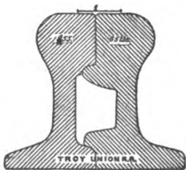
Compound Rail.
