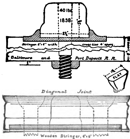
Thick Rectangular Rail, A. D. 1838.
