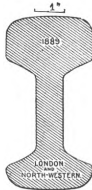
Bull-headed Rail.
