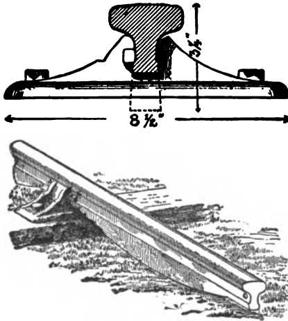
English Fish-belly Rail, New Jersey Railroad, A. D. 1882.
