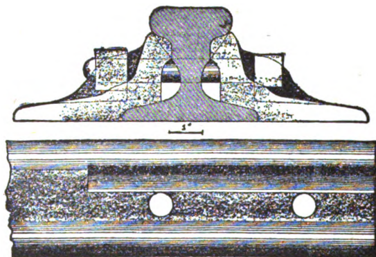
Erie Rill with ends stamped for Adams' Cast-Iron Bracket Splice, A.D. 1857.
