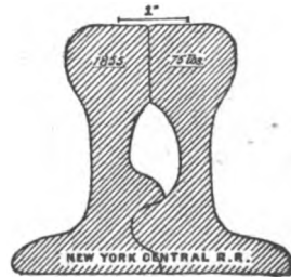
Compound Rail
