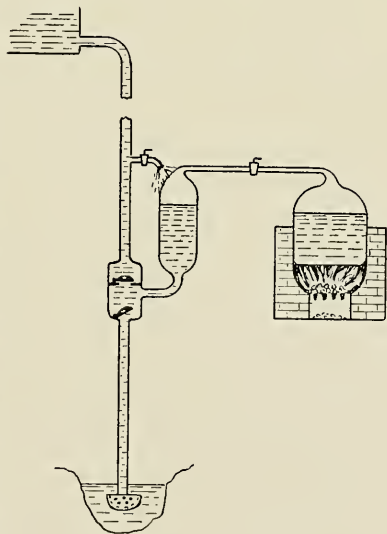
Savery's Engine
