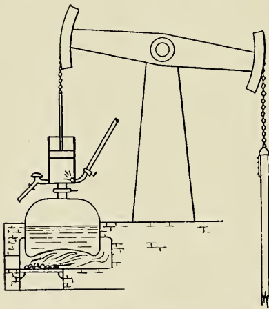
Newcomen's Engine
