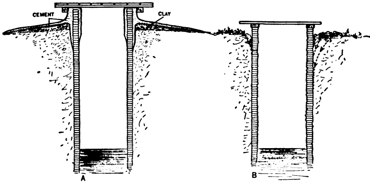
FIG. 156. B shows how surface water enters a well, carrying with it germs from the surface of the soil. A is a well arranged to keep out surface water and germs. The water must not be allowed to run down behind the wall, the platform should be double and water tight, and water should not be allowed to run back into the well around the pump.
