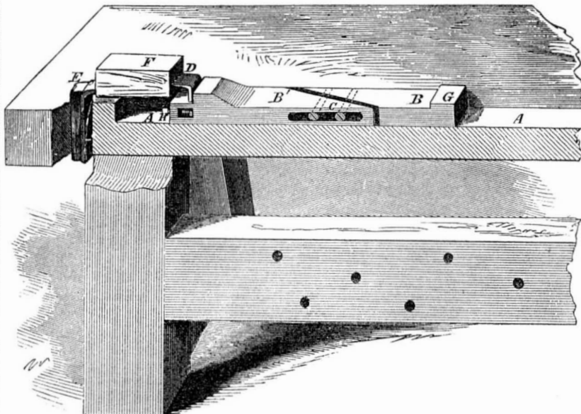
Improved Bench Hook.
