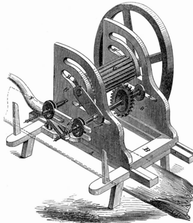
Machine for Boring Fence Posts.
