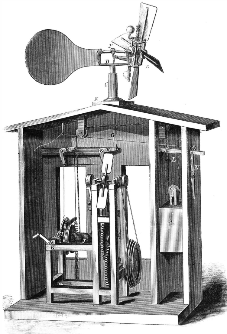
SMITH'S POWER ACCUMULATOR.
