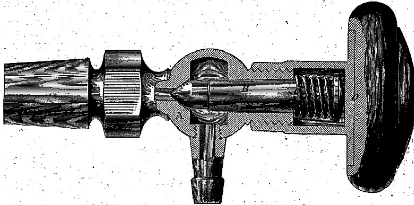
BROUGHTON'S GAGE COCK.
