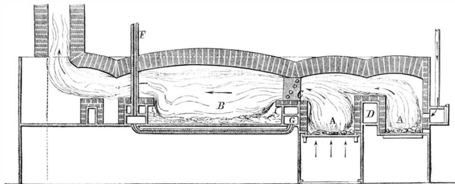
WILLIAMS'S FURNACE FOR PUDDLING IRON.
