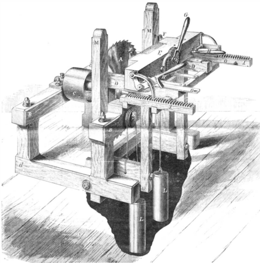
LOW'S SHINGLE AND BARREL-HEAD SAWING MACHINE.
