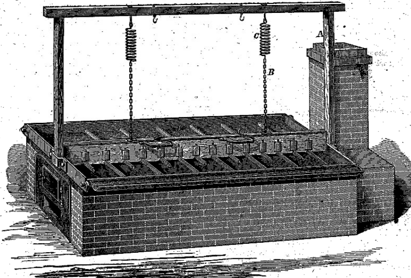
RIGGS'S SORGHUM EVAPORATOR.
