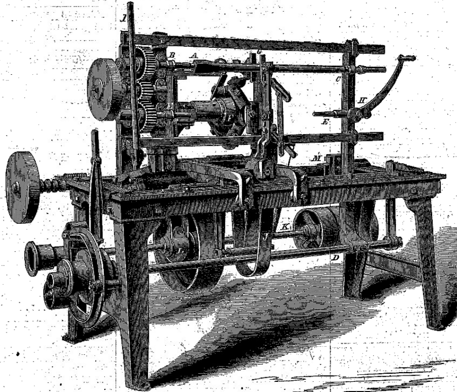
GLEASON'S SPOKE-TURNING LATHE.
