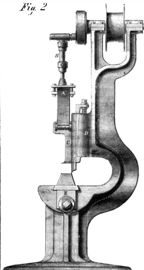
SHAW & JUSTICE'S DEAD-STROKE HAMMER.
