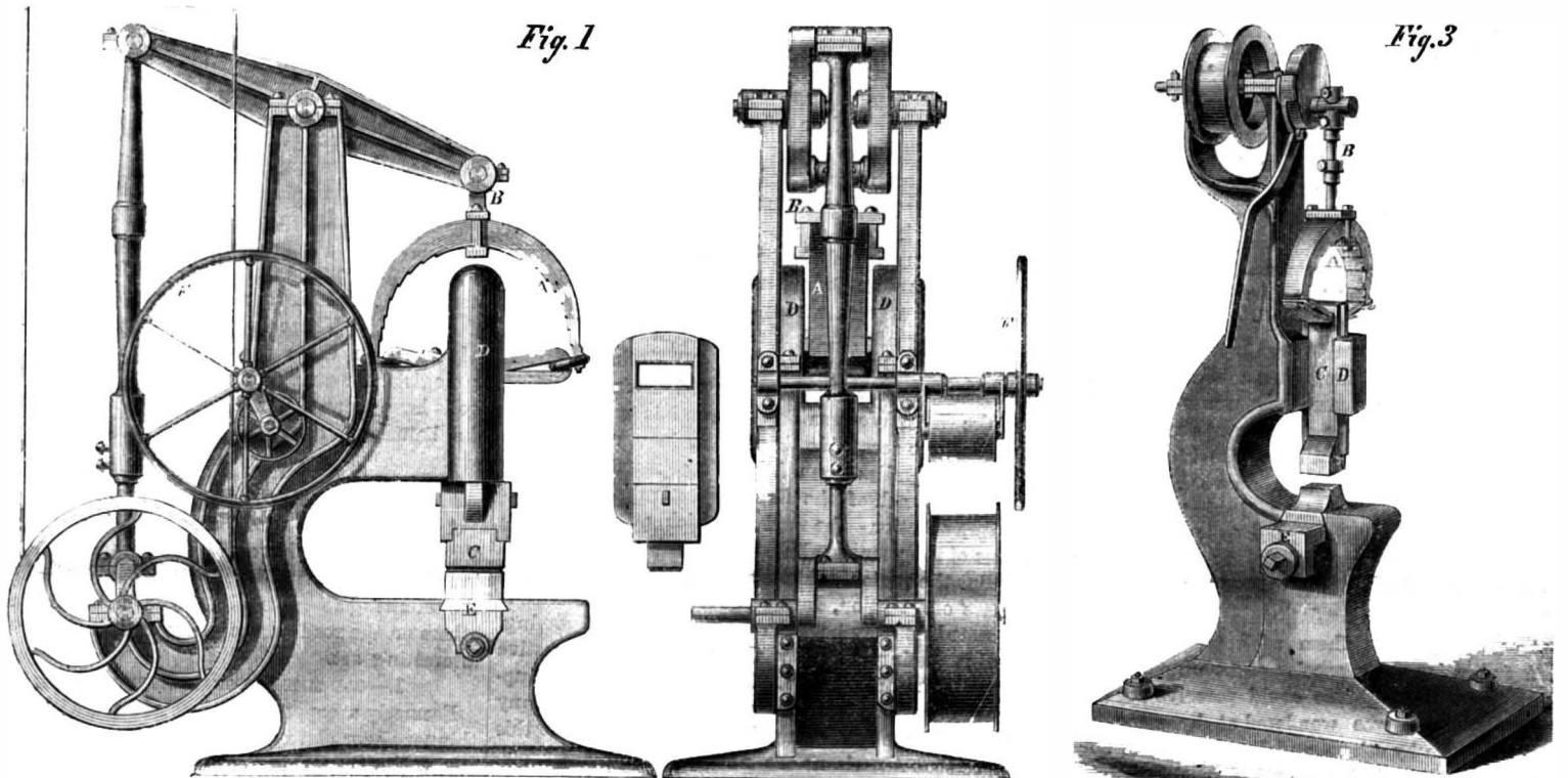
SHAW & JUSTICE'S DEAD-STROKE HAMMER.
