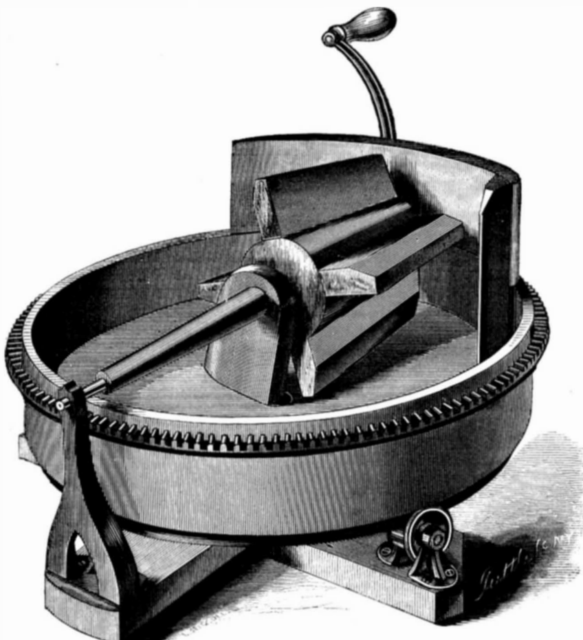
PEASE'S PATENT BUTTER-WORKER.
