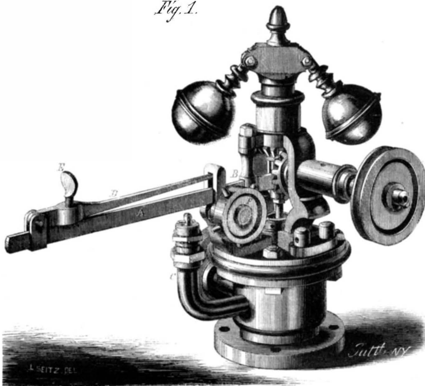
NUTZ AND ESTES' GOVERNOR AND STOP MOTION.
