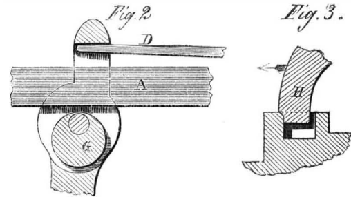
NUTZ AND ESTES' GOVERNOR AND STOP MOTION.
