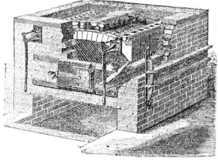
For Burning Pea and Dust Coal, and other fine material. Illustrated in Scientific American, issue of May 25, 1867.
